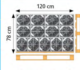
Europallet (80 x 120 cm) 13 containers per laag
