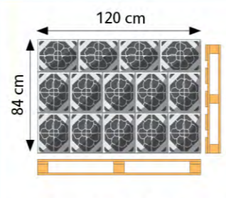
Europallet (80 x 120 cm) 14 containers per laag
