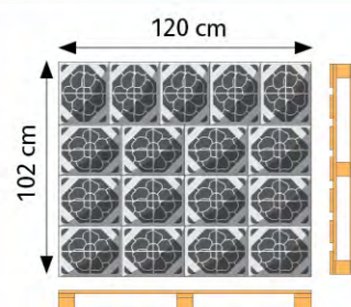
Blokpallet (100 x 120 cm) 17 containers per laag
