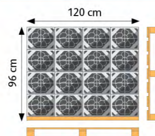
Blokpallet (100 x 120 cm) 16 containers per laag
