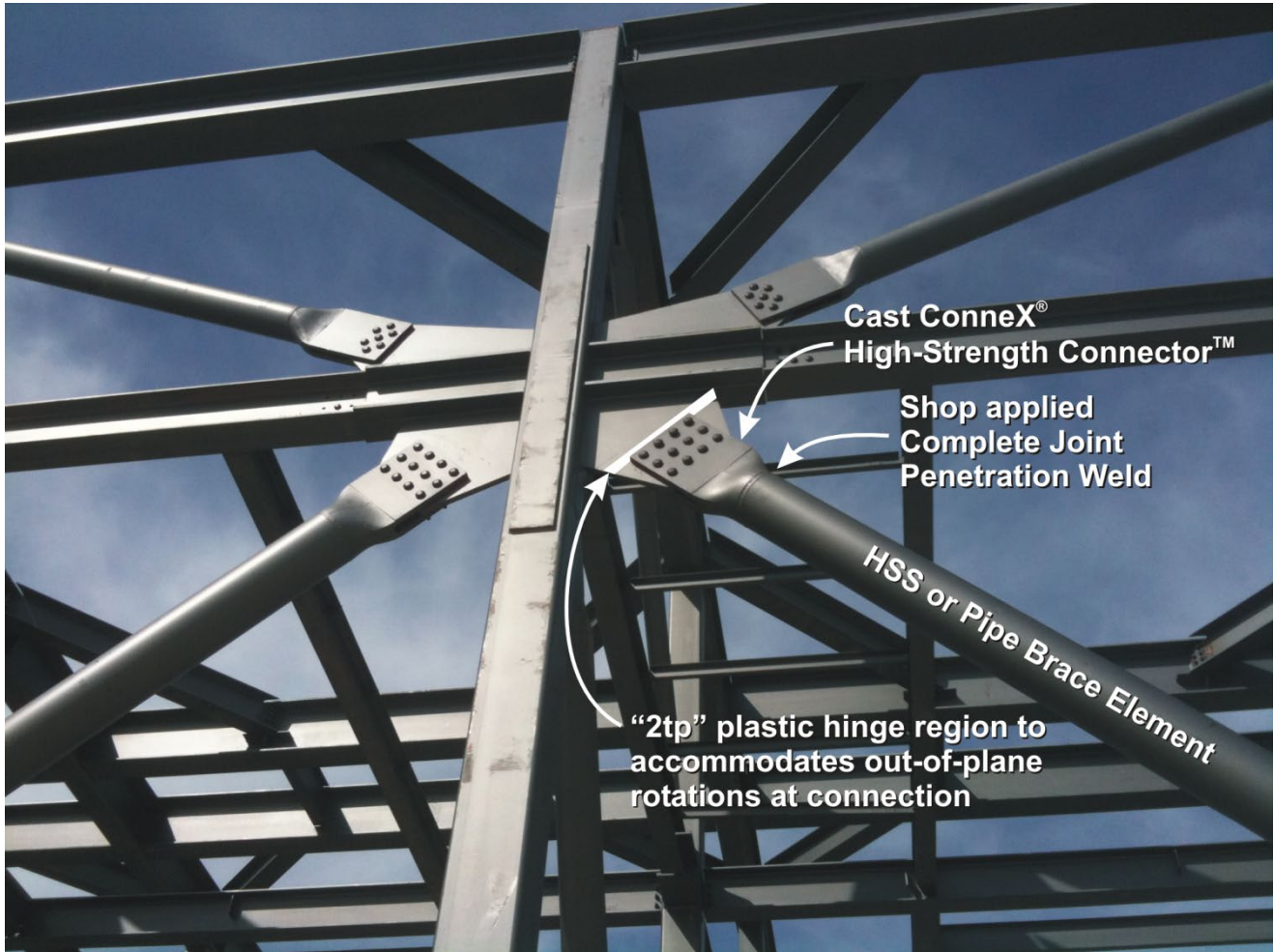
FIGURE 2—CAST CONNEX ® HIGH-STRENGTH CONNECTOR ™ SHOWN IN FIELD-BOLTED CONFIGURATION IN BRACED FRAME
