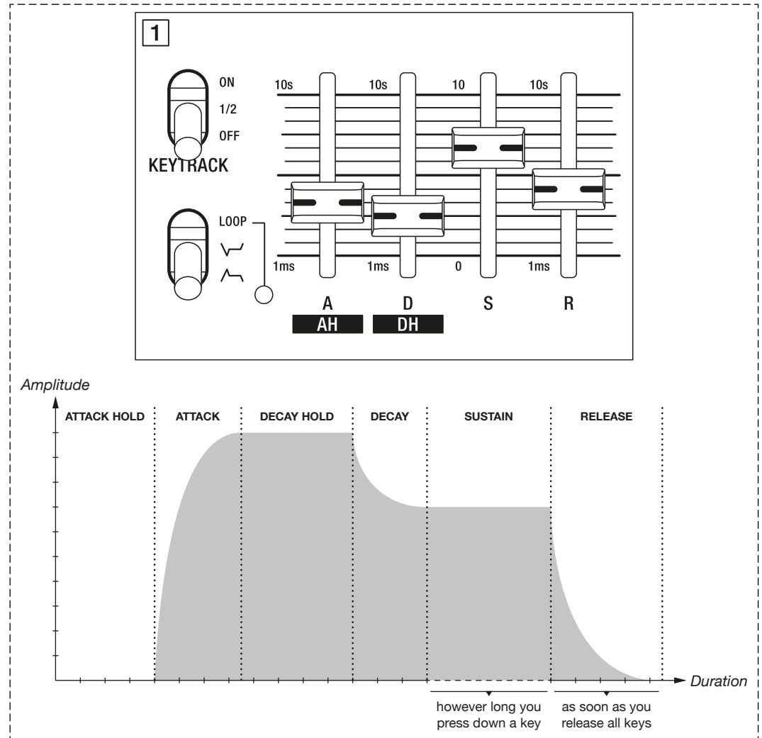
Envelope 1 setting and a diagram of the resulting envelope shape.
