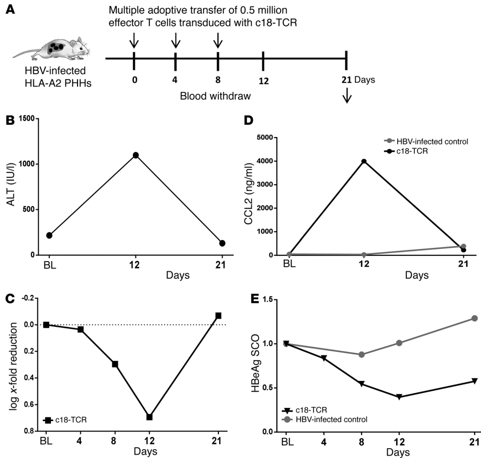
Figure 5. Adoptive transfer of mRNA HBV-specific TCR-electroporated T cells leads to temporary limited liver inflammation and cell damage. (A) Schematic representation of the experiment performed to assess the effect of multiple injections of electroporated effector T cells after treatment cessation both on inflammatory and virological parameters. (B) ALT levels were determined in 1 HBV-infected animal shortly before T cell injection (baseline) after receiving 3 injections of HBV-specific c18-TCR T cells (day 12) and 9 days after the last T cell injection (day 21). (C) Longitudinal changes in viremia relative to baseline were determined at 4, 8, 12, and 21 days after the first T cell transfer as depicted in A. (D) Serum protein levels of CCL2 were determined in both 1 HBV-infected control mouse (gray) and 1 mouse receiving multiple T cell injections (c18-TCR), and that was monitored for 21 days. (E) Longitudinal changes in levels of circulating HBeAg were determined by ELISA in the same mice described in D.
