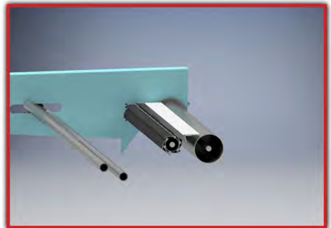
A driven push out/lifter roller at the discharge end of the machine helps to gradually push out stuck product without damage.
