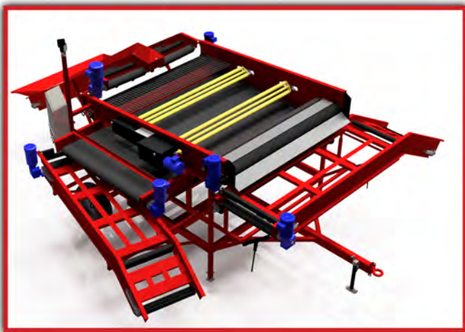
Dual independently driven shaker/agitators.
