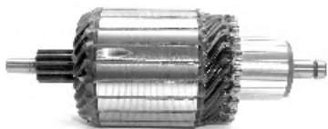
IM 3130 12 V 1.8 Kw Replacing: 1004011211, 234166 Servicing: 0001110132, F000AL0108 Slots:23 Teeth:11 O.D.59,0 L. 160,0
