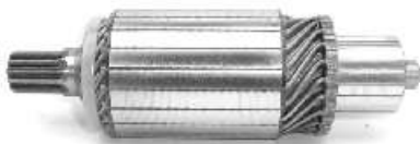
IM 3085 24 V 6.5 Kw Replacing: 132009700X0, 138964 Servicing: 03506020110, 03506020118, 03506020149, 03506020233, 03506020248, 03506020258, 03506020261, ... Slots:21 Teeth:12 O.D.65,0 L.206,5
