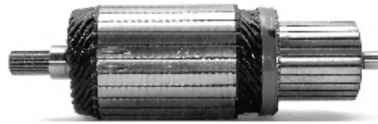
IM 3170 12 V 2.0 Kw Replacing: 028200-6860, 139148, 28160-54380 Servicing: 228000-2120, 228000-2680, 228000-2690, 228000-2700, 228000-2980, 228000-3840, 228000-3850, ... Slots:27 Teeth:21 O.D.50,45 L.159,7
