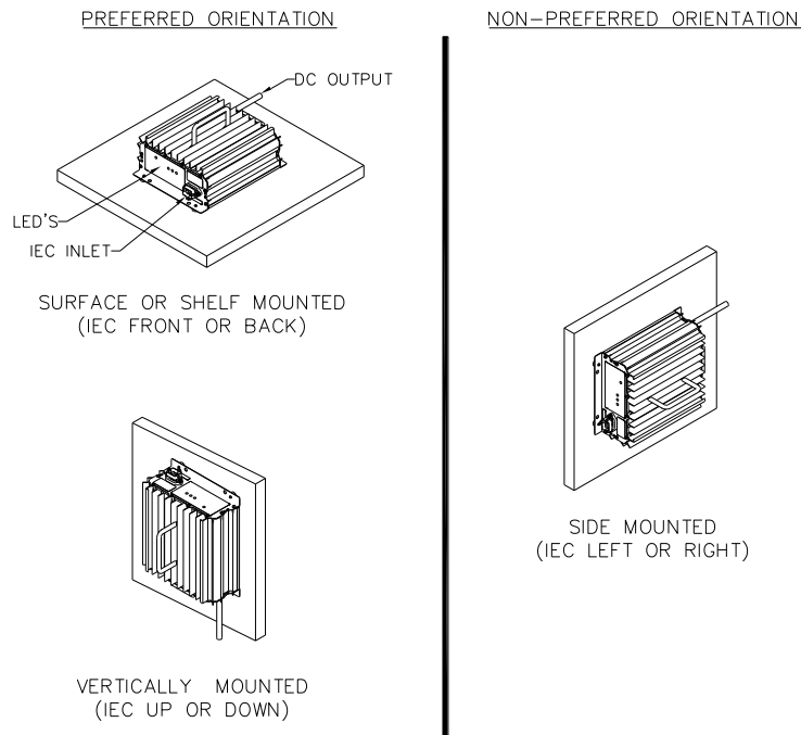
Figure 2-1: Charger Mounting Recommendations
