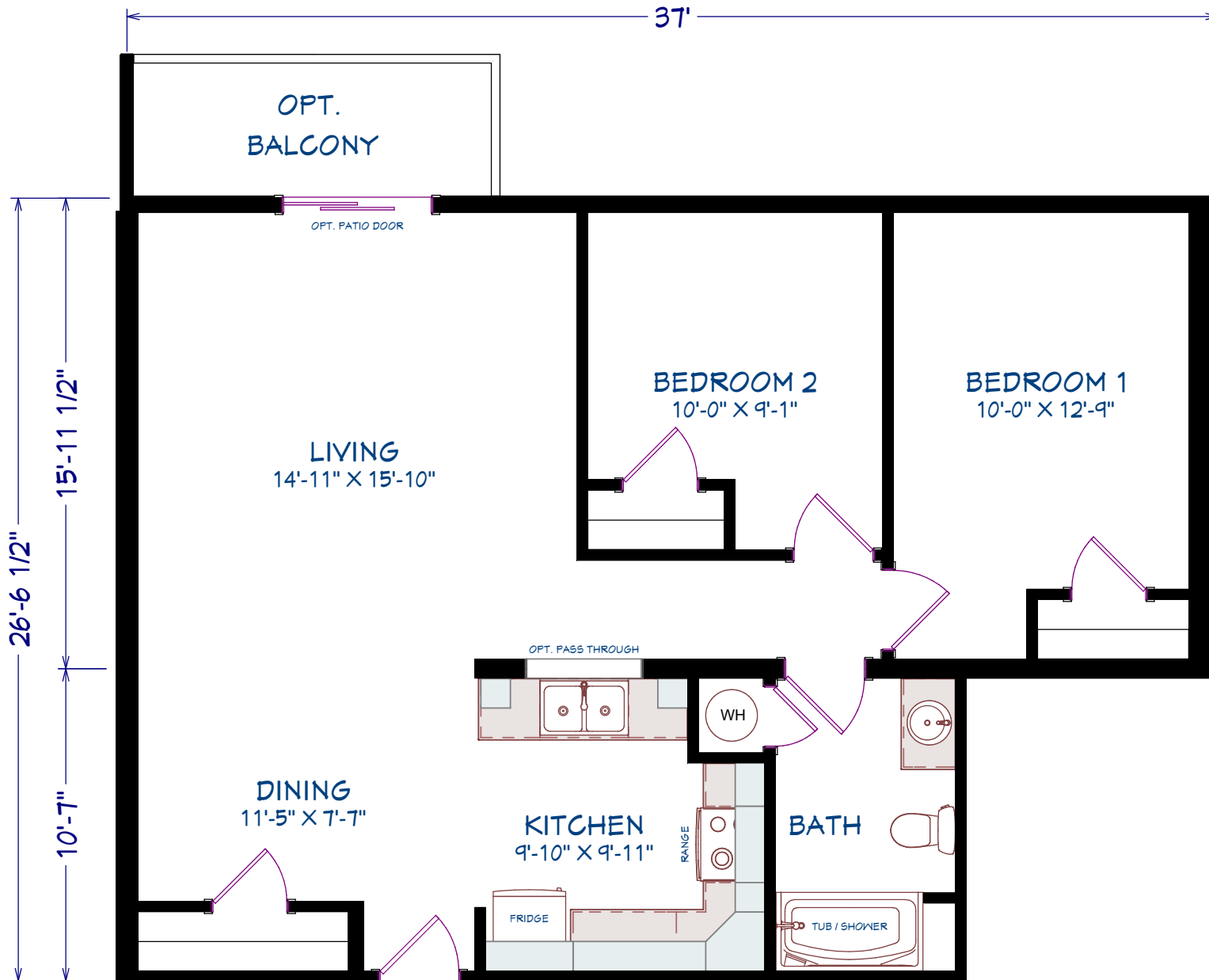
CUSTOM LEVEL MULTI UNIT, 2 BEDROOM UNIT 902 SQ FT
