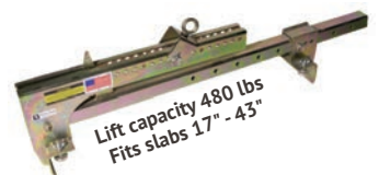
Large Slab Lifter
