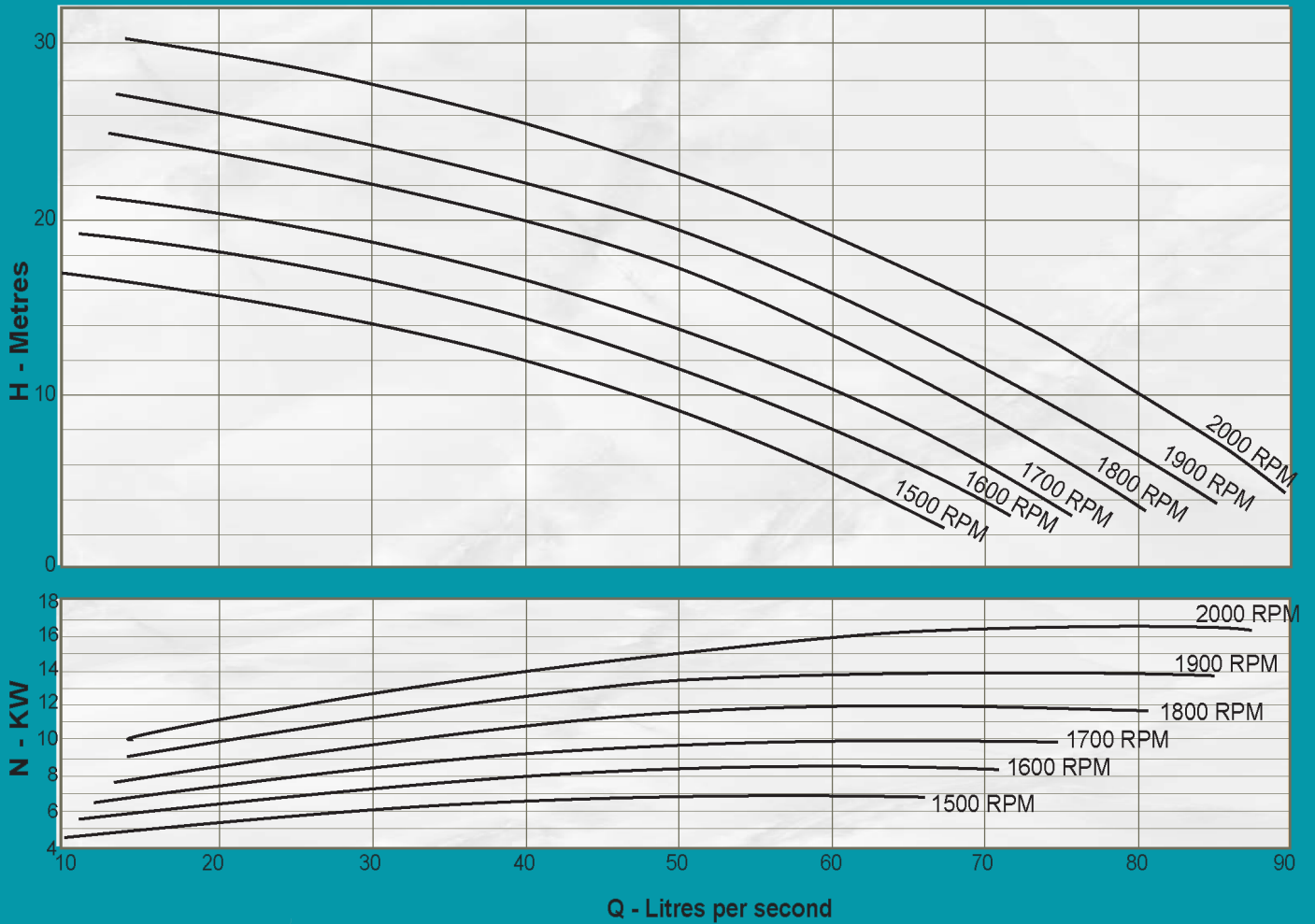
FSR150 Pump Curve
