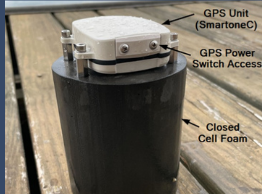
Trajectory sensors with GPS and floatation system.
