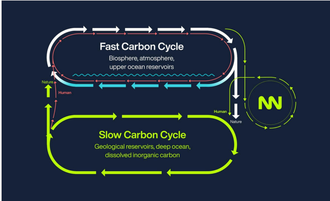
Figure 1: The fast and slow carbon cycles.
