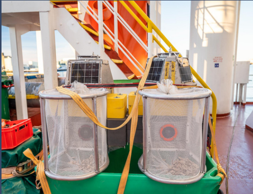
Open ocean observation platform with integrated sensor suites, macroalgae growth image capture, OAE dissolution rates, sinking location, wave and wind action, and more.
