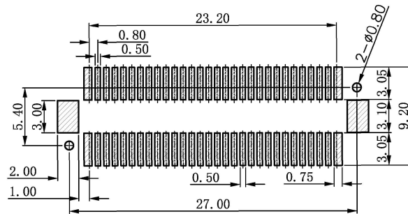
RECOMMENDED PCB LAYOUT TOLERANCE: ±0.05mm
