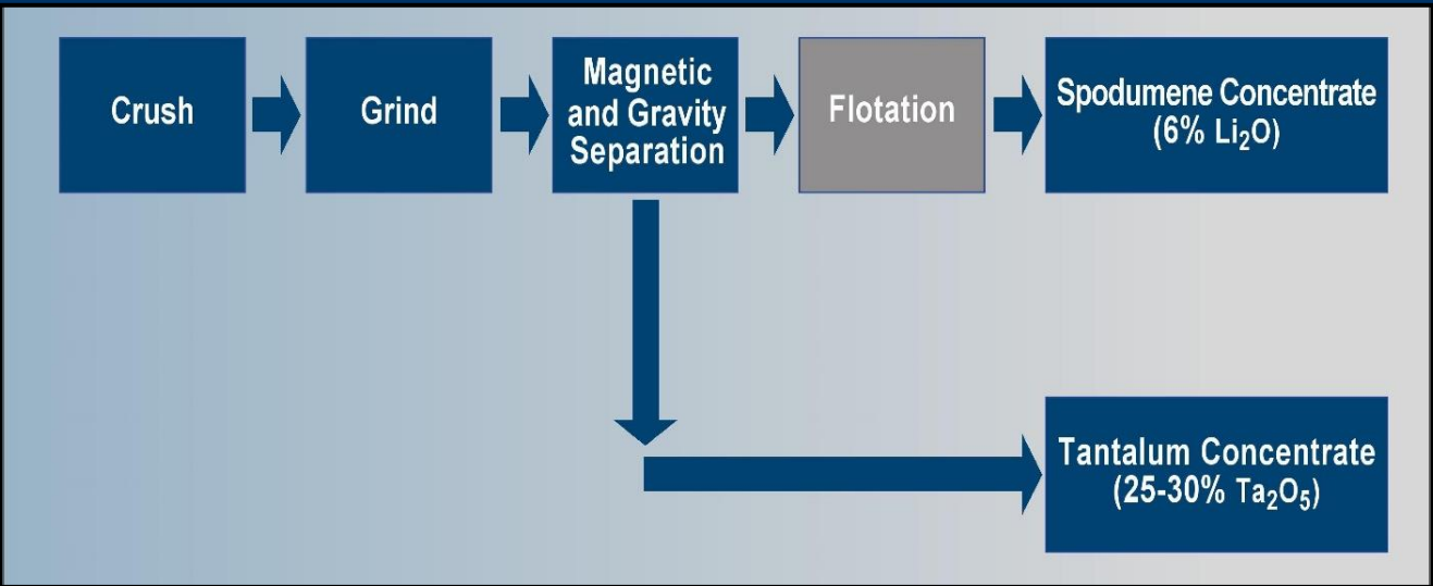
Proposed Simplified Whole Ore Flotation Flowsheet
