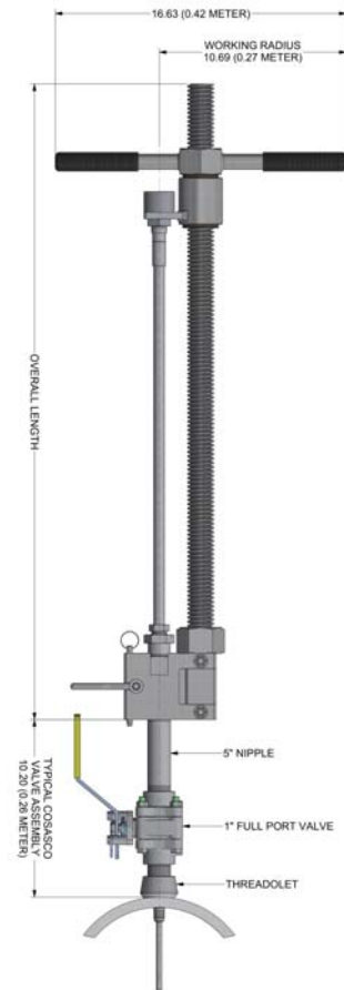
*CUSTOMER CONFIGURATION MAY VARY. 24" RETRACTOR FOR 18" & 24" PROBES - 35" (0.89 METER) 36" RETRACTOR FOR 18" TO 36" PROBES - 47" (1.20 METER)
