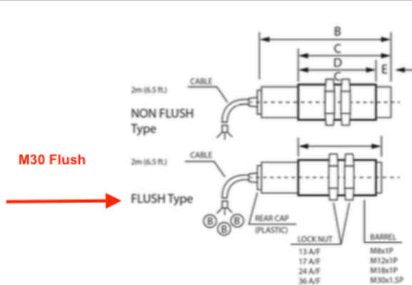
* All dimensions in mm, NB-Nickel Brass, SS-Stainless Steel, TS-Triple Sense Stainless Steel
