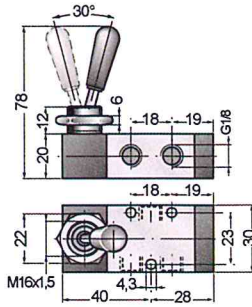
VALVE / VALVOLA 3/2
