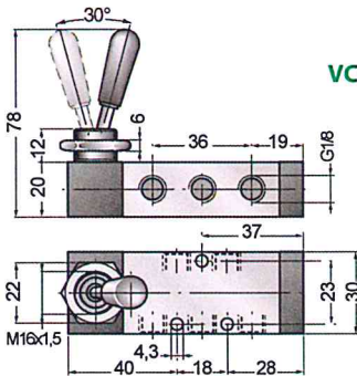
VALVE / VALVOLA 5/2 - 5/3
