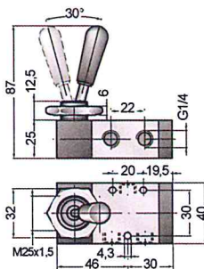
VALVE / VALVOLA 3/2
