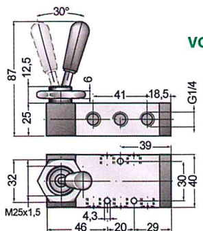
VALVE / VALVOLA 5/2 - 5/3
