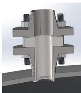
Top Hat Assembly in Tank Service
