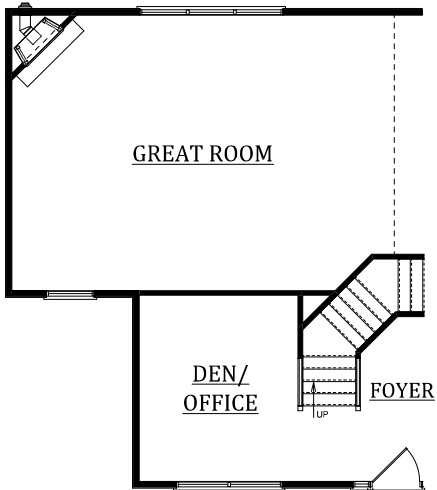
OPTIONAL 1ST FLOOR PLAN 1,418 Sq. Ft.
