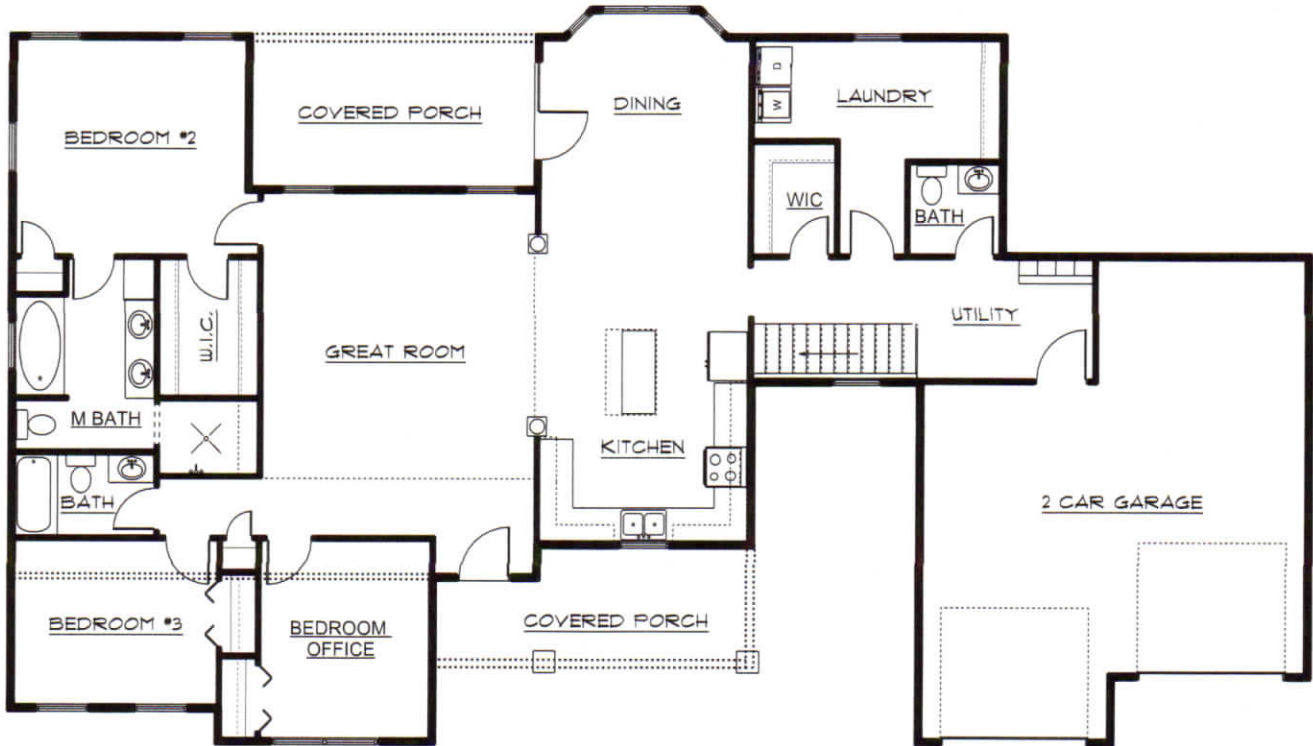
FLOOR PLAN
