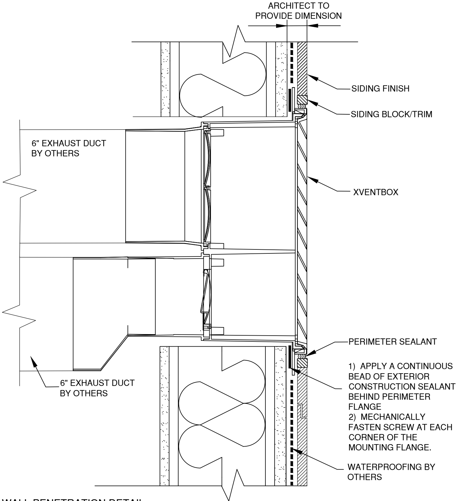
WALL PENETRATION DETAIL
