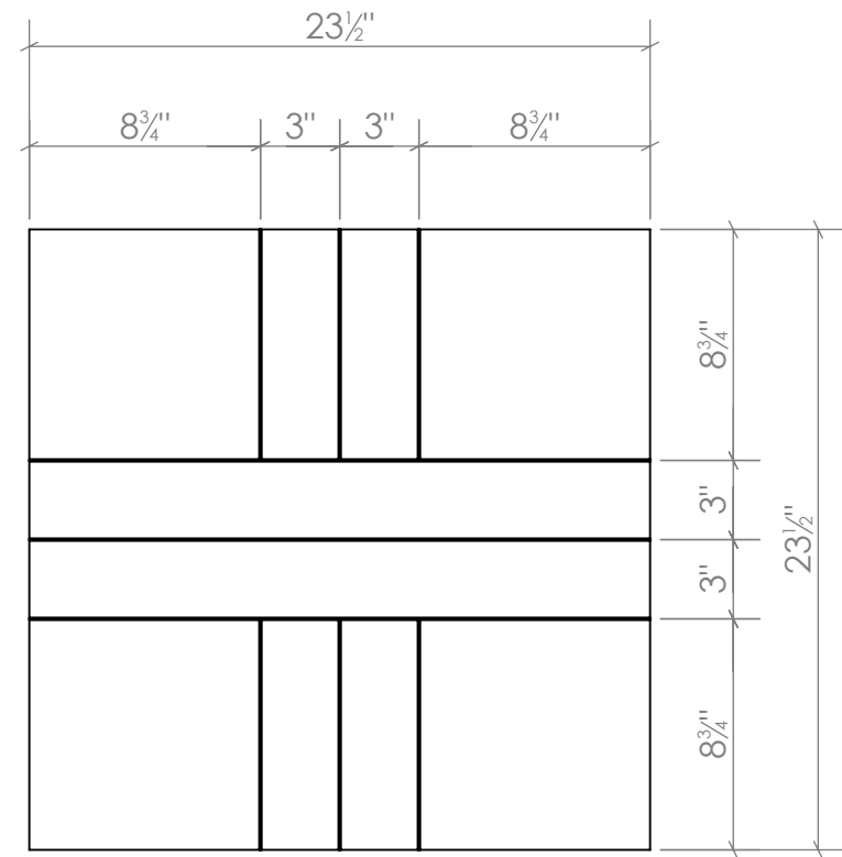
2 SHEET 3 X SECTION WALL PANEL - ELEVATION
