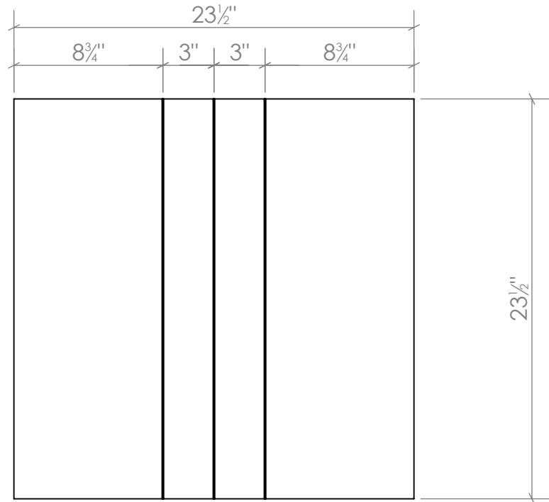
4 SHEET 1 STRAIGHT WALL PANEL - ELEVATION
