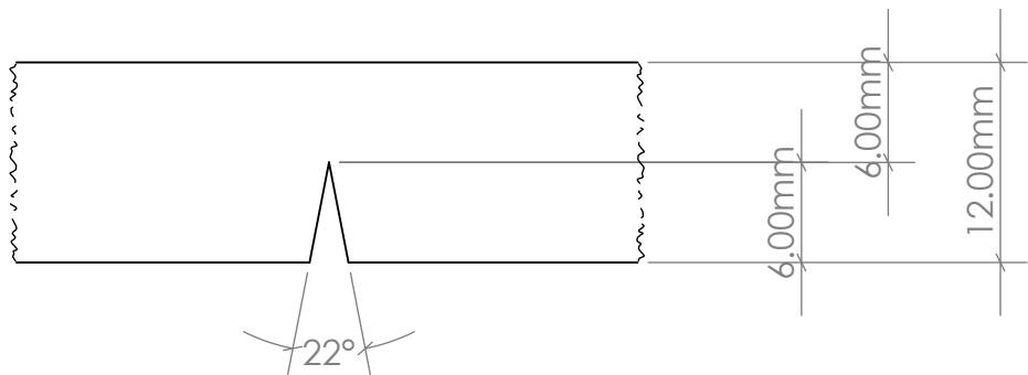
2 SHEET 1 DETAIL 2/SHEET 1 - V CUT SCALE - 2:1
