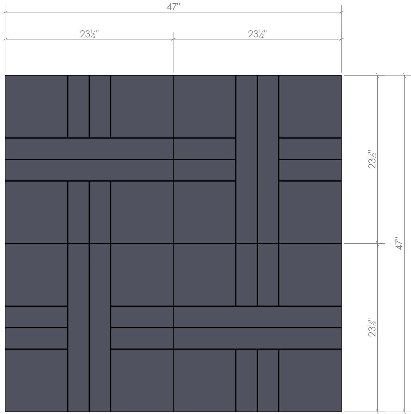
1 SHEET 3 X SECTION WALL PANEL ASSEMBLY - ELEVATION
