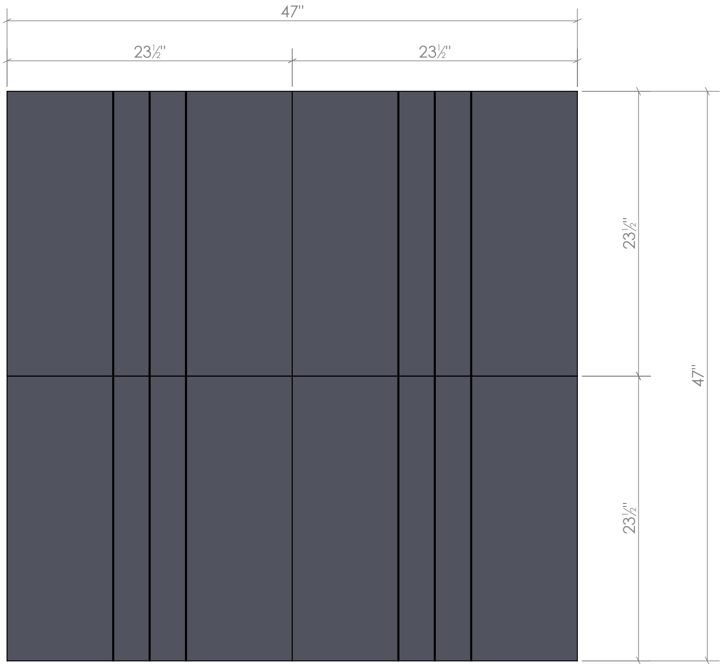
1 SHEET 1 STRAIGHT WALL PANEL ASSEMBLY - ELEVATION
