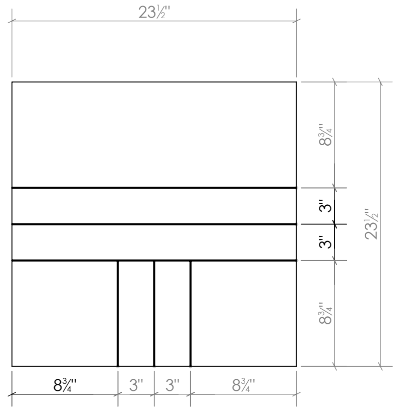
2 SHEET 4 T SECTION WALL PANEL - ELEVATION
