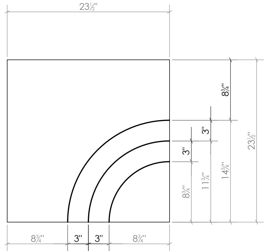
2 SHEET 5 CURVE WALL PANEL - ELEVATION
