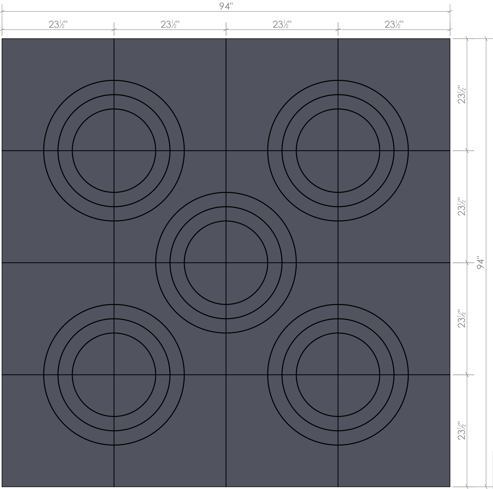
DOUBLE CURVE WALL PANEL ASSEMBLY - ELEVATION
