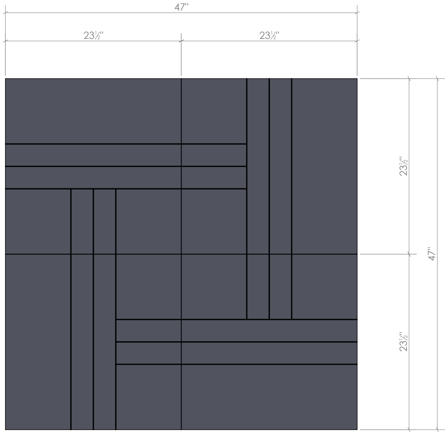
1 SHEET 4 T SECTION WALL PANEL ASSEMBLY - ELEVATION
