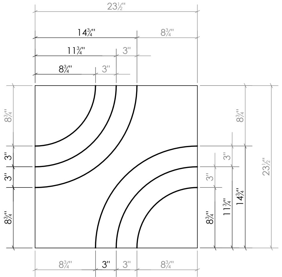
DOUBLE CURVE WALL PANEL - ELEVATION SCALE - 1:8
