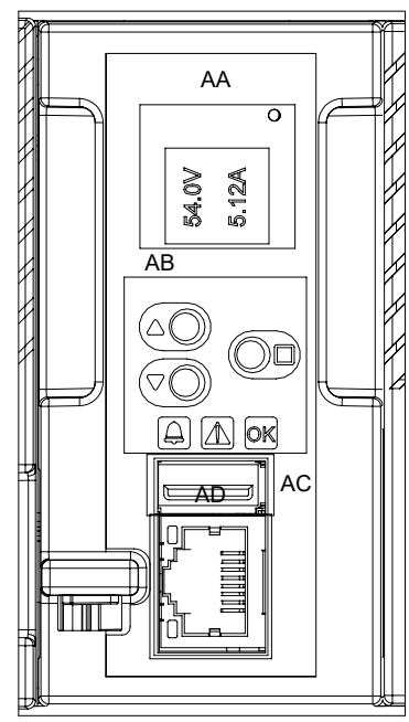
CORDEX CXCM1 HP SYSTEM CONTROLLER DETAIL A
