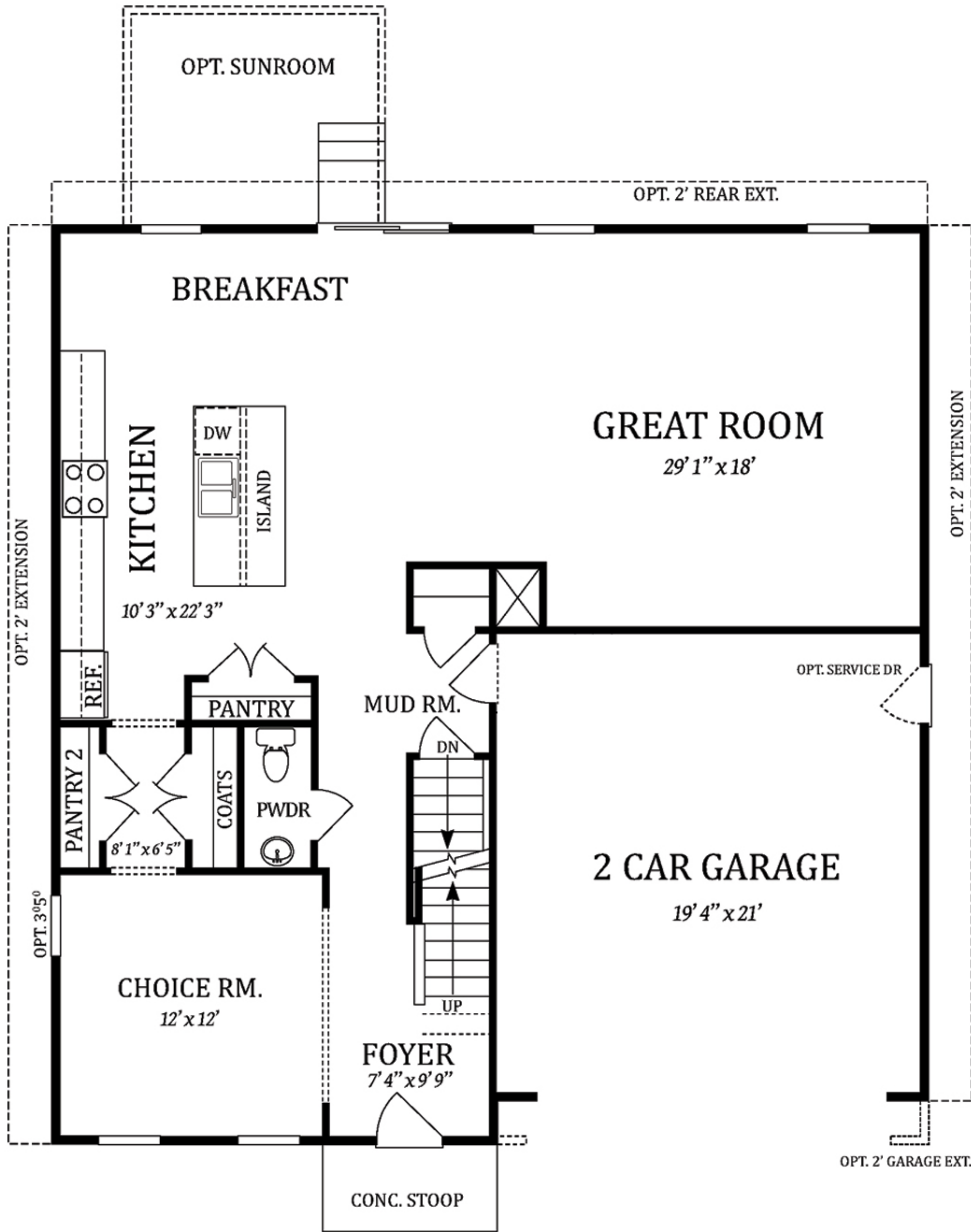
FIRST FLOOR PLAN 9' CEILING
