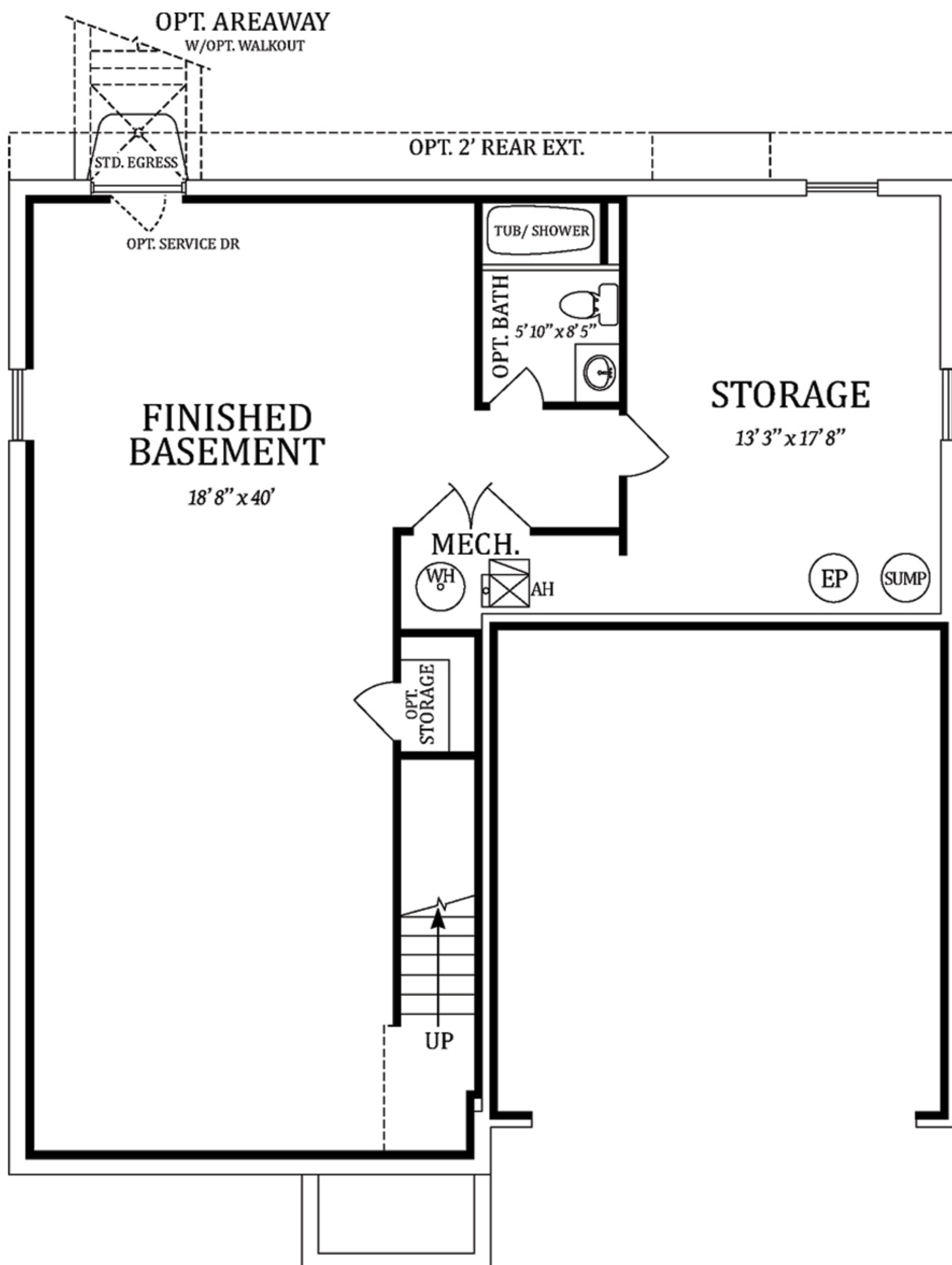
OPT. FINISHED LOWER LEVEL FLOOR PLAN 8' CEILING
