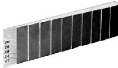
10 Step Aluminium Wedge with Wire Backer
