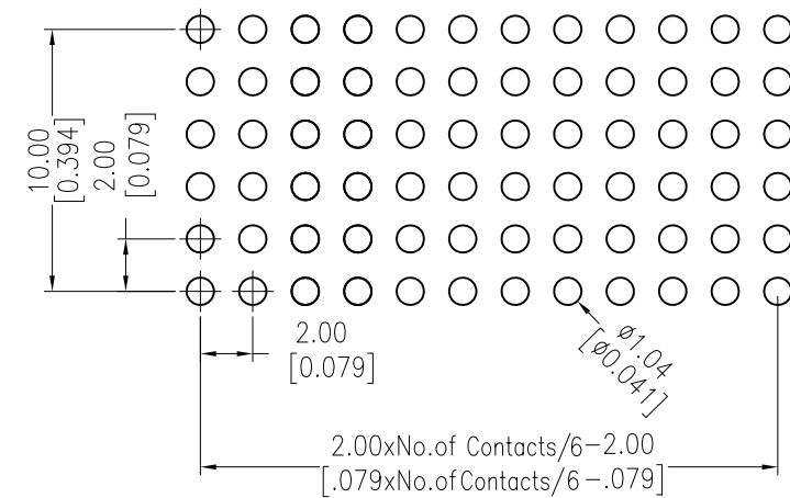
Recommended P.C.B Layout(Top Side) (PCB BOARD TOLERANCE±0.05)
