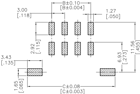
RECOMMENDED PCB LAYOUT TOLERANCE IS ±0.05
