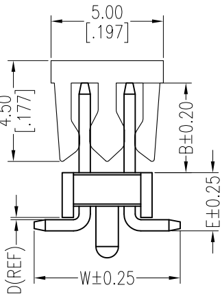
TYPE 2 WITH POST
