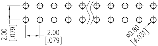
Recommended P.C.B Layout(Top Side) (PCB BOARD TOLERANCE±0.05)
