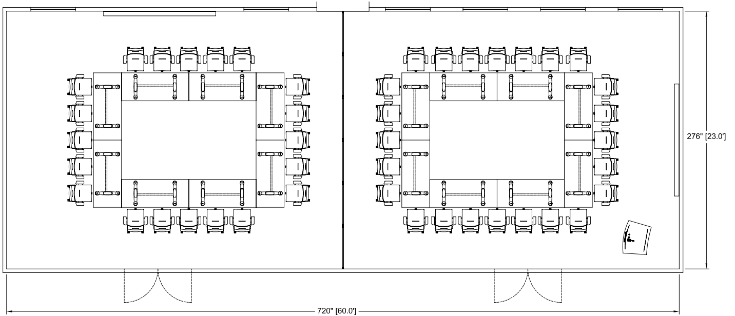
ROOM1-LAYOUT C2
