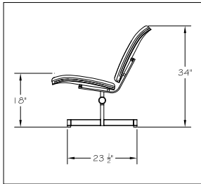
Side elevation
