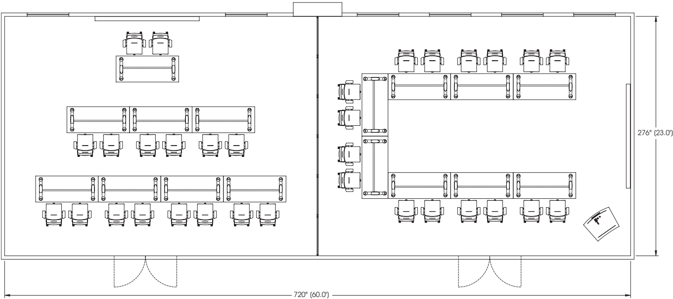
ROOM1-LAYOUT A4
