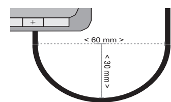
Fig. 16: Minimum cable bend radius
