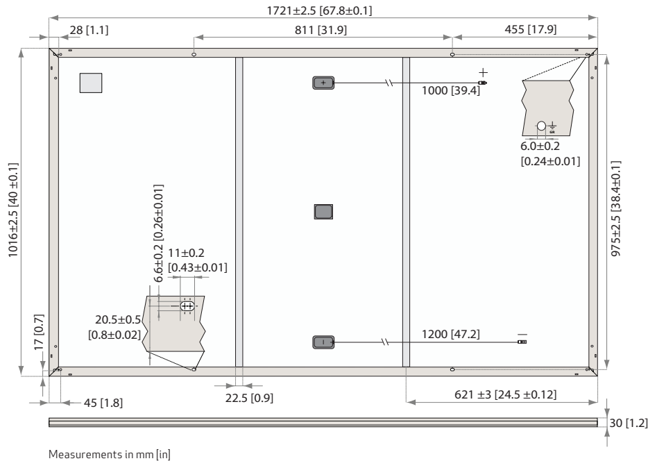
Fig. 19: Panel dimensions: REC Alpha Black Series
