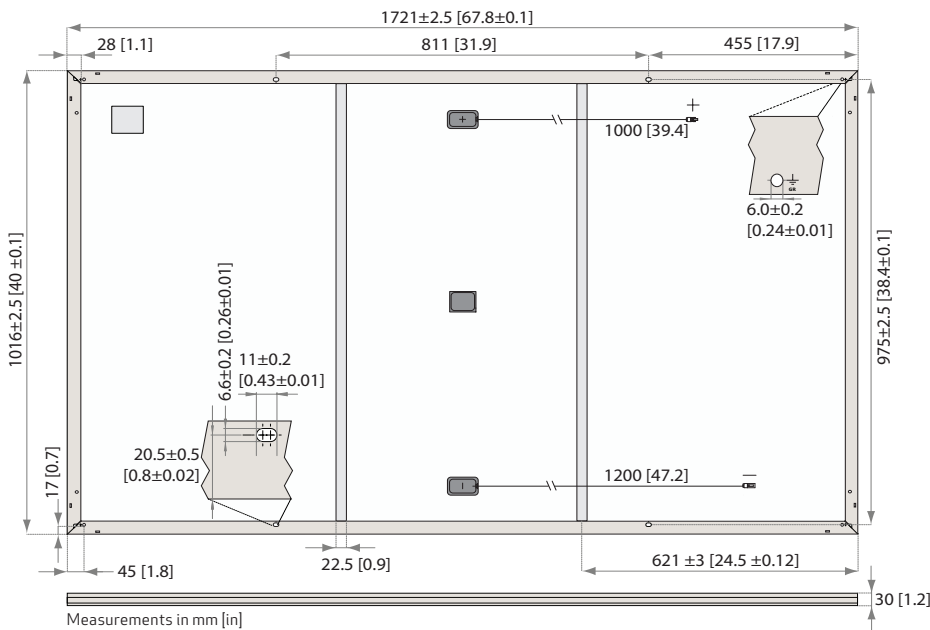
Fig. 18: Panel dimensions: REC Alpha Series
