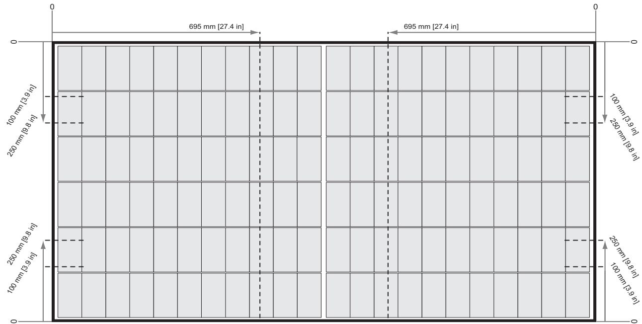
Fig. 4: Clamping of REC Alpha Series panels with rails parallel to long side of the panel
