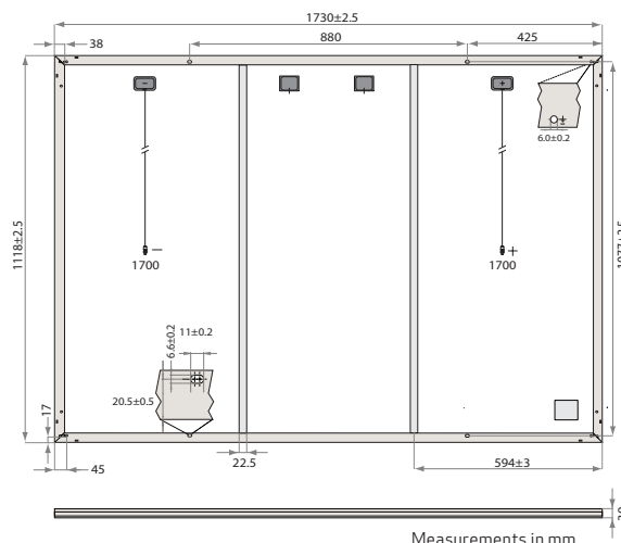
Fig. 21: Panel dimensions: REC Alpha Pure-R Series
