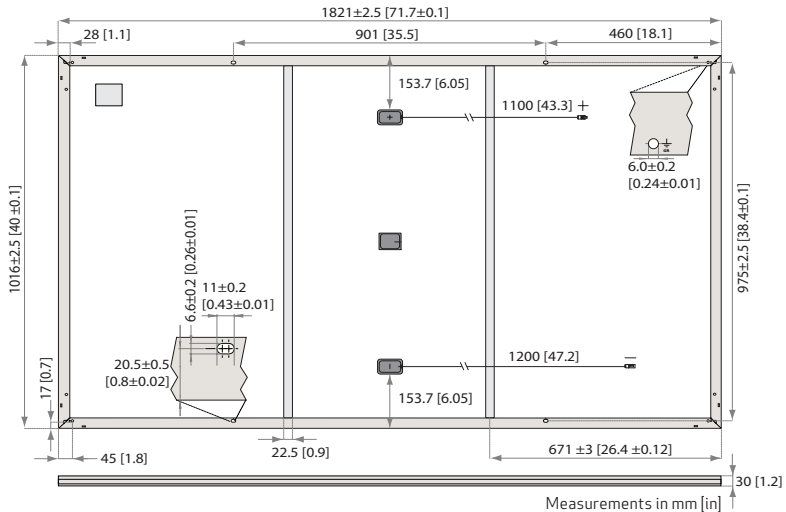
Fig. 20: Panel dimensions: REC Alpha Pure Series
