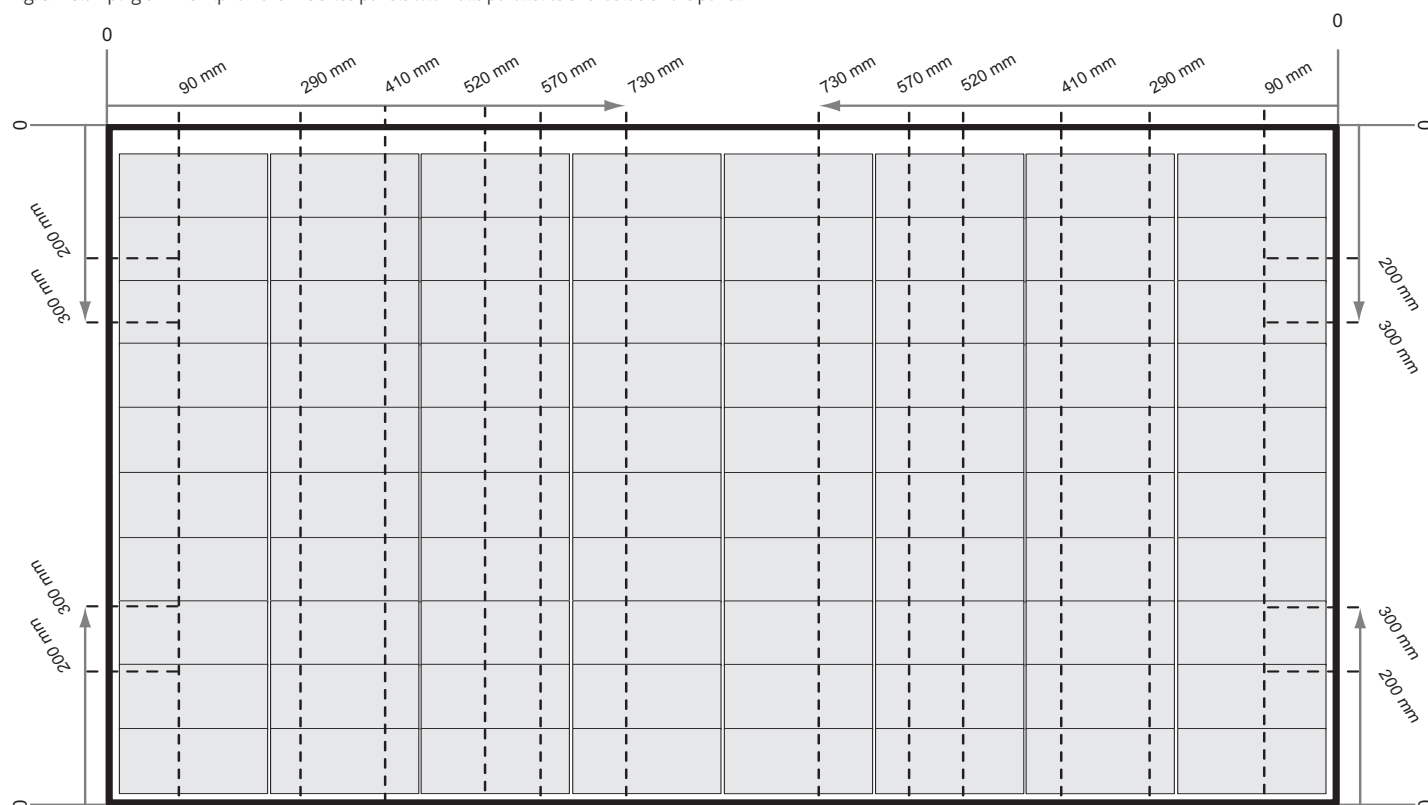
Fig. 9: Clamping of REC Alpha Pure-R Series panels with rails parallel to short side of the panel
