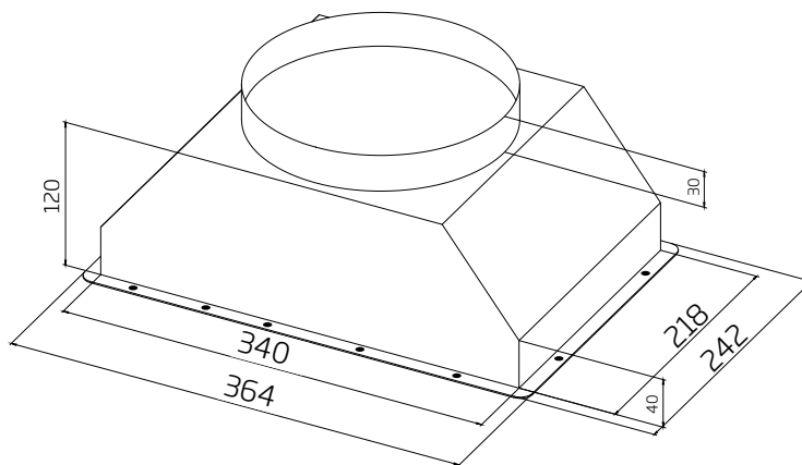
Dual 150mm to 200mm adaptor
