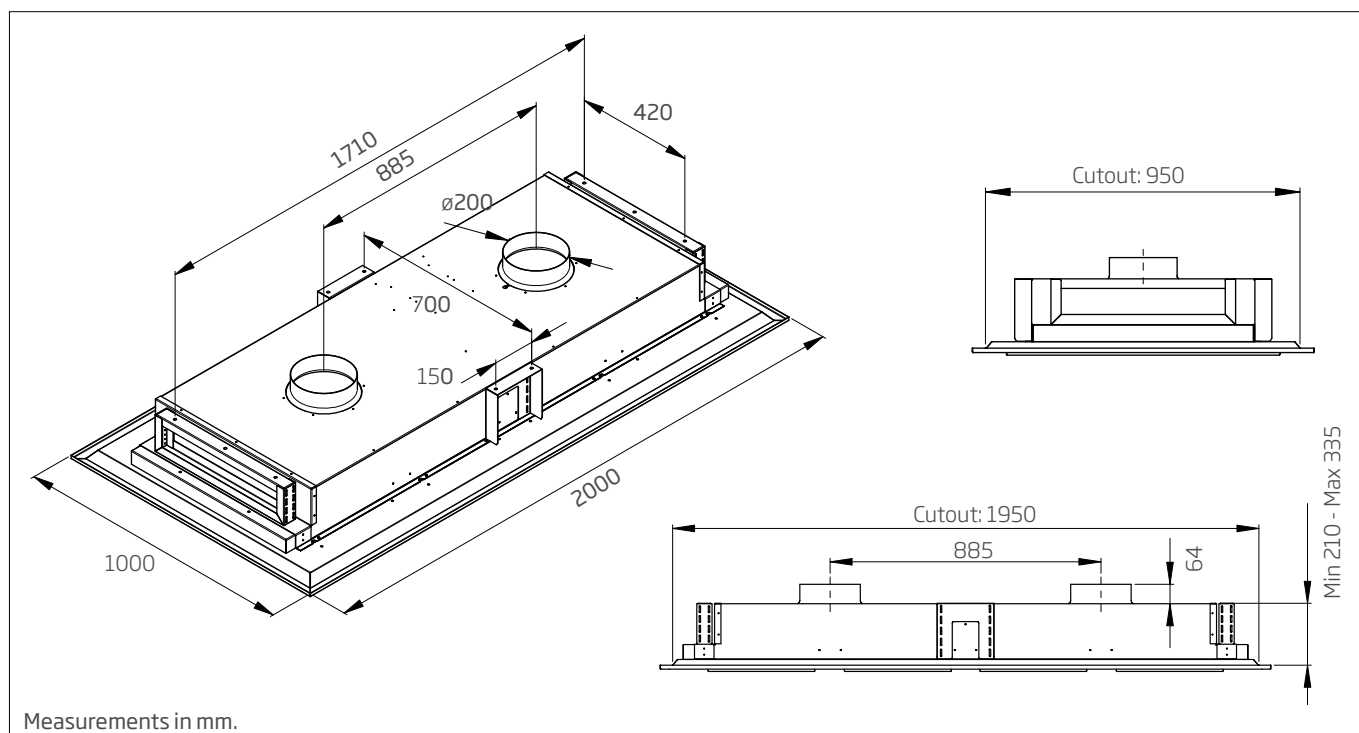
Figure 2 Cut Out Dimensions for CC-INARTS
