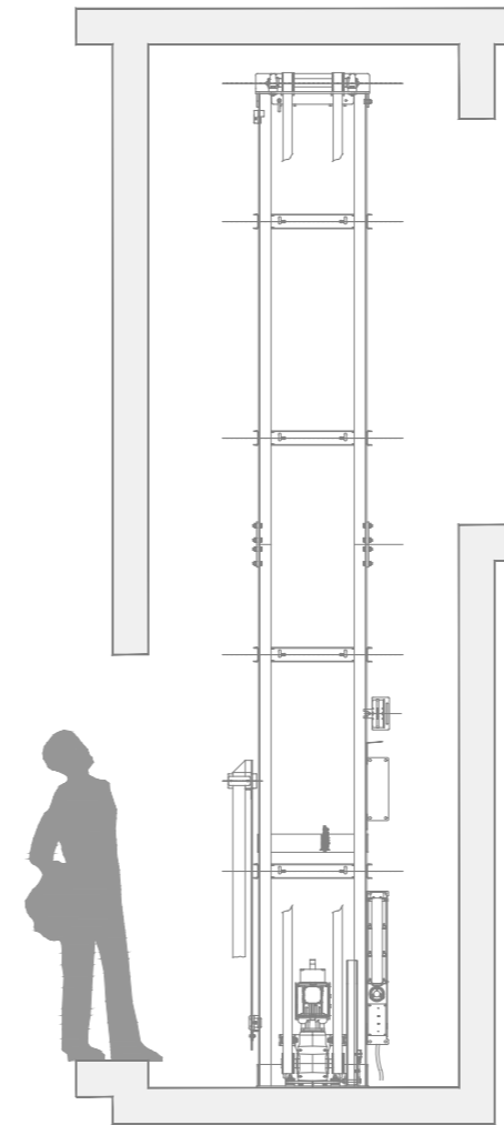
TRACTION DRIVE SYSTEM
