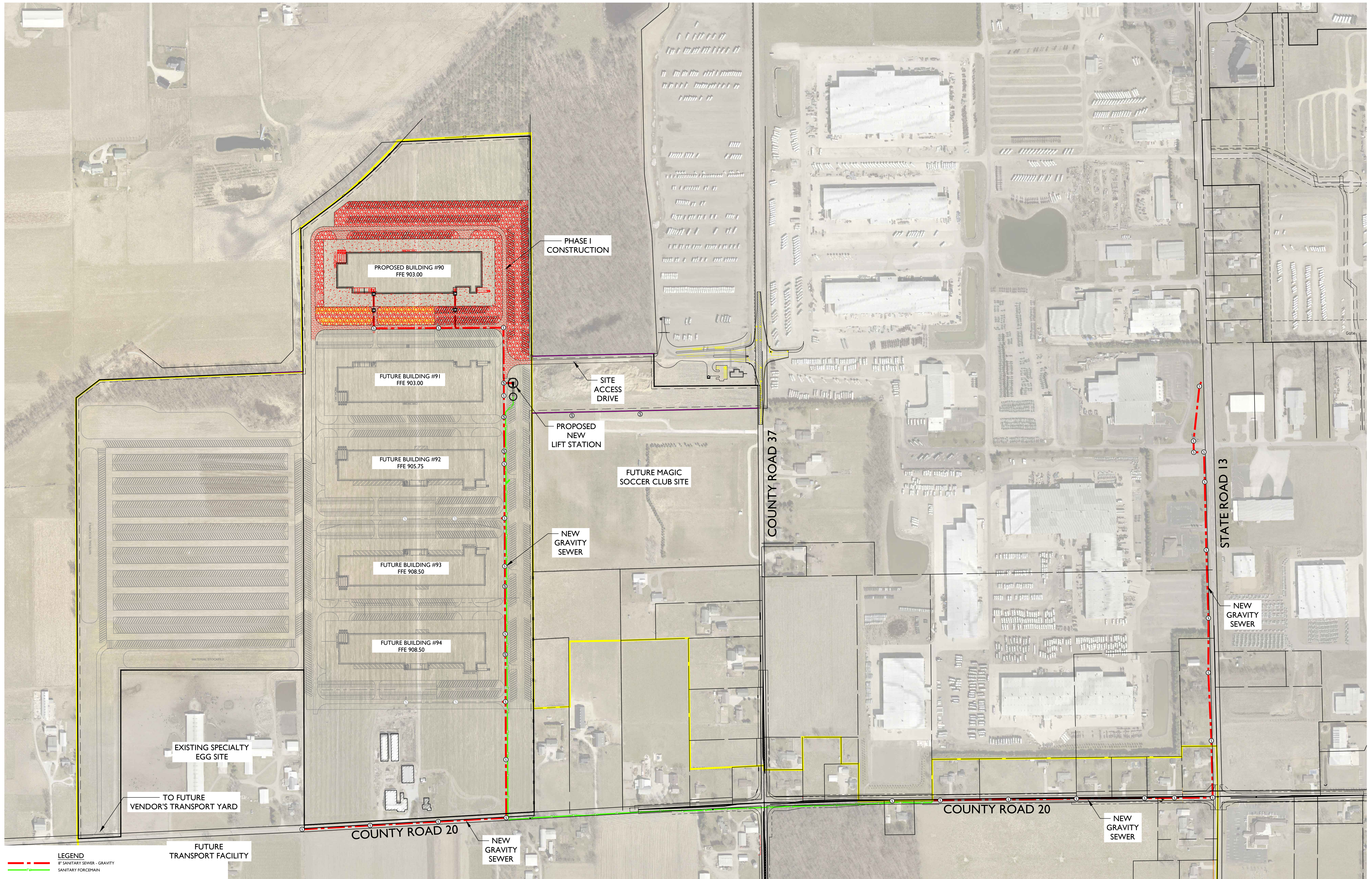
TOWN OF MIDDLEBURY FIGURE 3A - SANITARY SEWER IMPROVEMENTS
