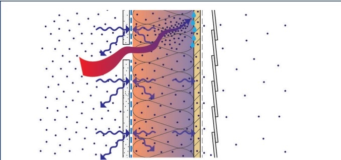
1.B) Air leakage by-passing the vapor barrier will still condense on the backside of the sheathing in cold climates.
