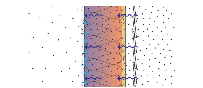
Humid outdoor air diffuses through the wall assembly until it reaches the cooler drywall. The cooler air is unable to store as much water as the warmer exterior air and so the relative humidity increases, but the water vapor concentration remains the same. If the RH exceeds certain thresholds, condensation and/or potential mold growth could happen.
