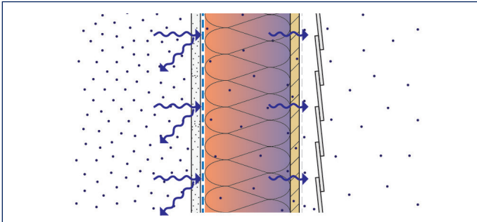
1) Vapor diffusion is blocked from flowing into the wall assembly and condensing within it using a vapor barrier at the interior side in cold climates.
