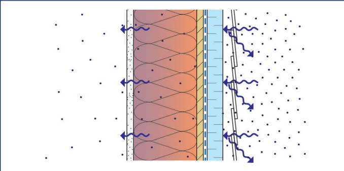
1.A) Vapor diffusion flow through a wall is restricted with the use of a vapor retarding insulation layer (shown as exterior insulation in this image).
