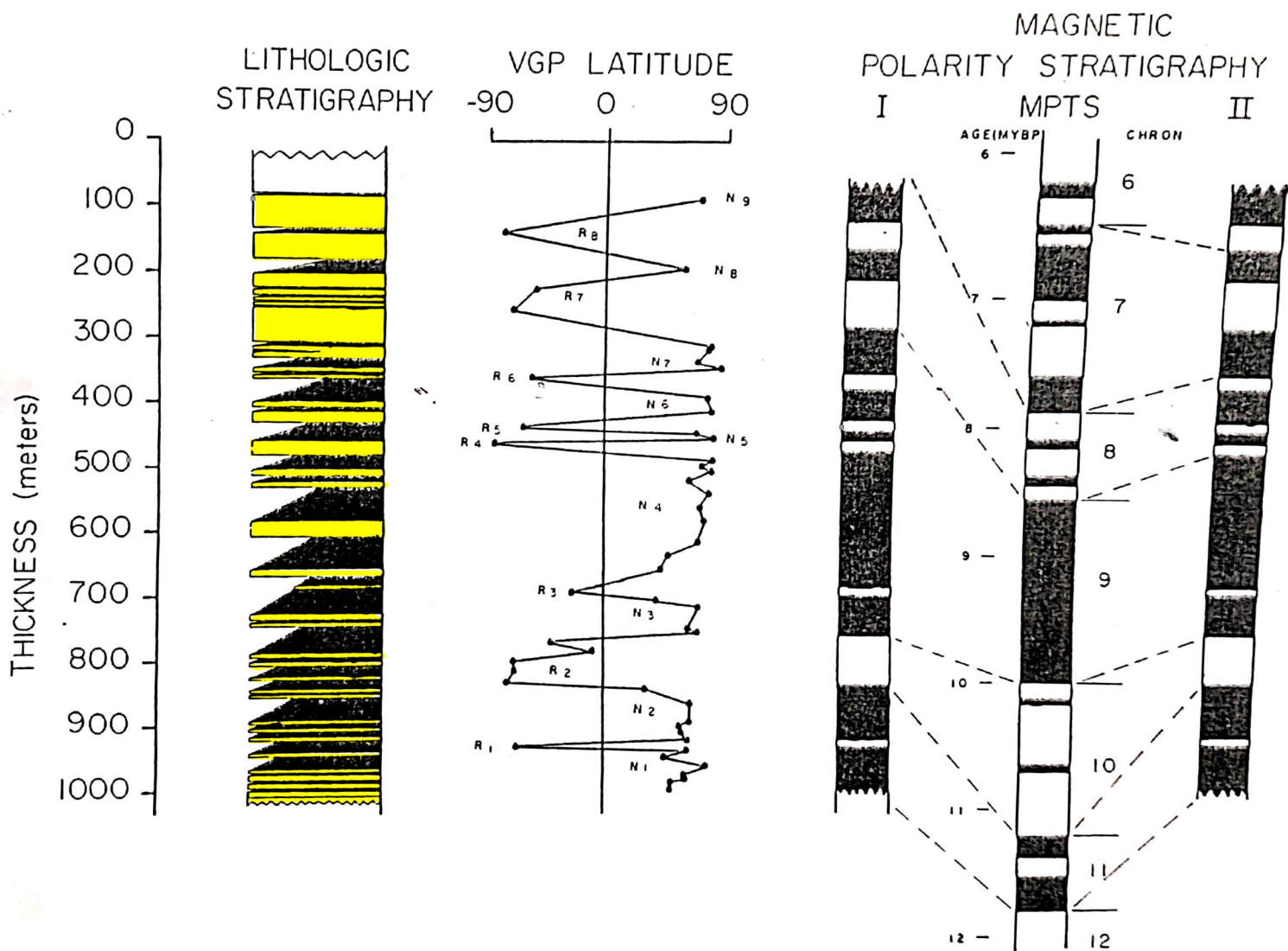
Fig. 7. Plot of VGP latitude versus stratigraphic thickness. Plotting conventions are same as for Fig. 4.
