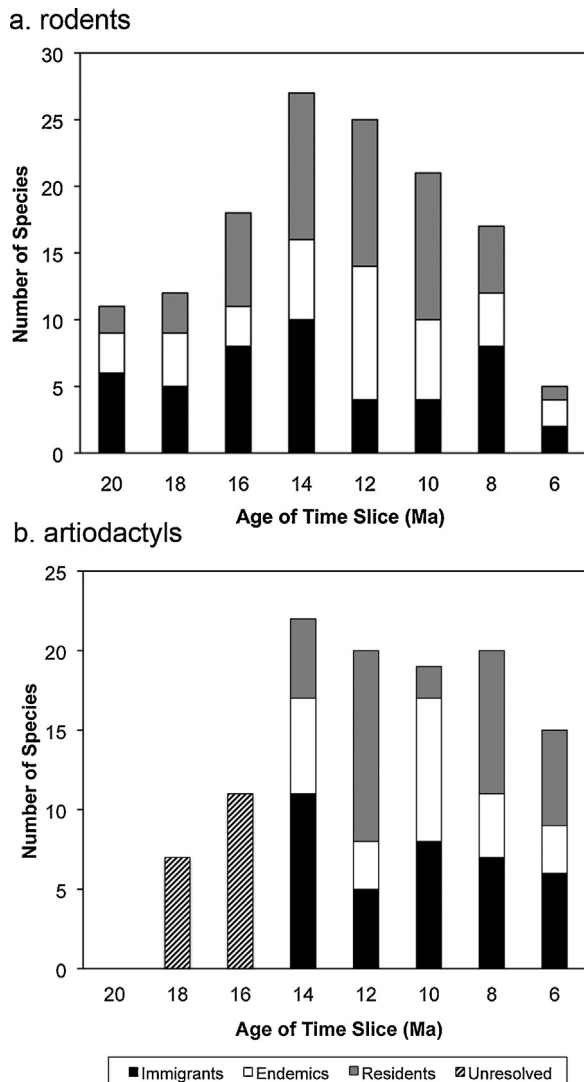
Fig. 3. Rodents (a) and artiodactyls (b) recorded at time slices centered at 2 m.y. intervals. Species are classified as residents or newcomers, newcomers being of endemic or immigrant origin. These categories are defined in Flynn et al. (2014), from which the figure is modified. Older and younger rodents and artiodactyls are known but are not part of the analysis; artiodactyl diversity for the 16 and 18 Ma time slices is indicated, but relationships to younger species are unresolved (cross hatch symbol). The underrepresented oldest and youngest time slices are affected by the few known localities of those ages (see Fig. 2).
