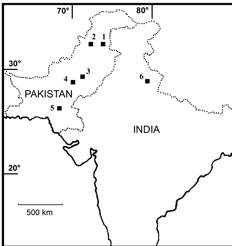
Fig. 1. Major collecting areas of the Indian Subcontinent. 1, Potwar Plateau (Barry et al., 2002, 2013; Flynn et al., 1995); 2, Indus Valley (De Bruijn et al., 1981; Munthe et al., 1979; Wessels et al., 1982); 3, Zinda Pir Dome (Antoine et al., 2013; Lindsay et al., 2005); 4, Bugti, Baluchistan (Welcomme et al., 2001); 5, Manchar Formation, Sindh (Wessels, 2009); 6, Siwalik Hills, one of many areas in India (Patnaik, 2013).
