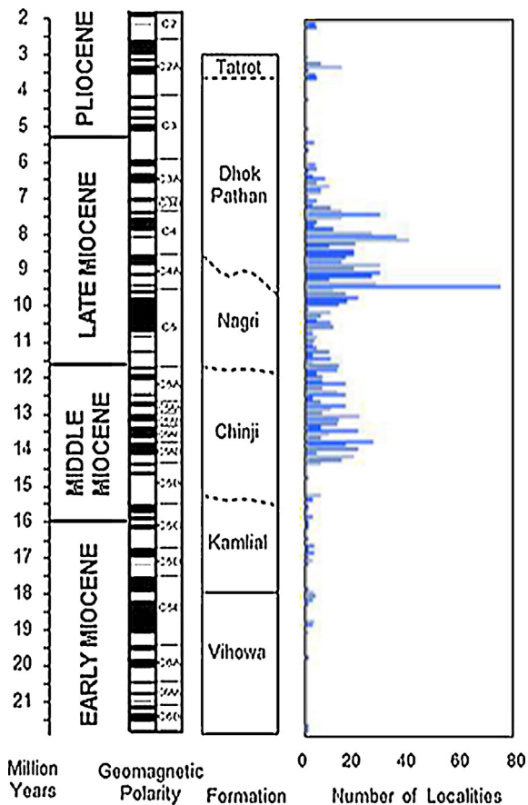
Fig. 2. Distribution through time of numbers of localities documented primarily in the Potwar Plateau, supplemented by information from the Upper Siwaliks of Pakistan, especially near Tatrot, and the Vihowa Formation of the Zinda Pir Dome. Geomagnetic Chrons are plotted on the time scale of Gradstein et al. (2004) . This figure illustrates the uneven record, number of sites being a proxy for recorded fossils, but localities differ in productivity. On the right, numbers of localities resolved to 10^5 years are plotted in 100,000 year bins.
