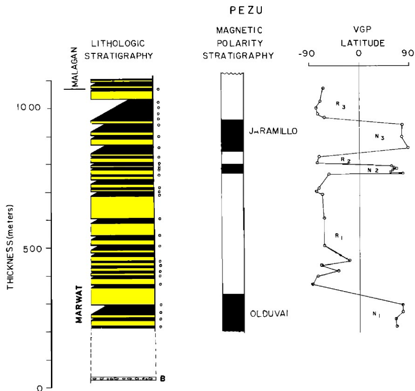
Fig. 9. Pezu Pass. Plot of VGP latitudes against stratigraphic thickness. The plotting convention is the same as Figures 6 and 8.
