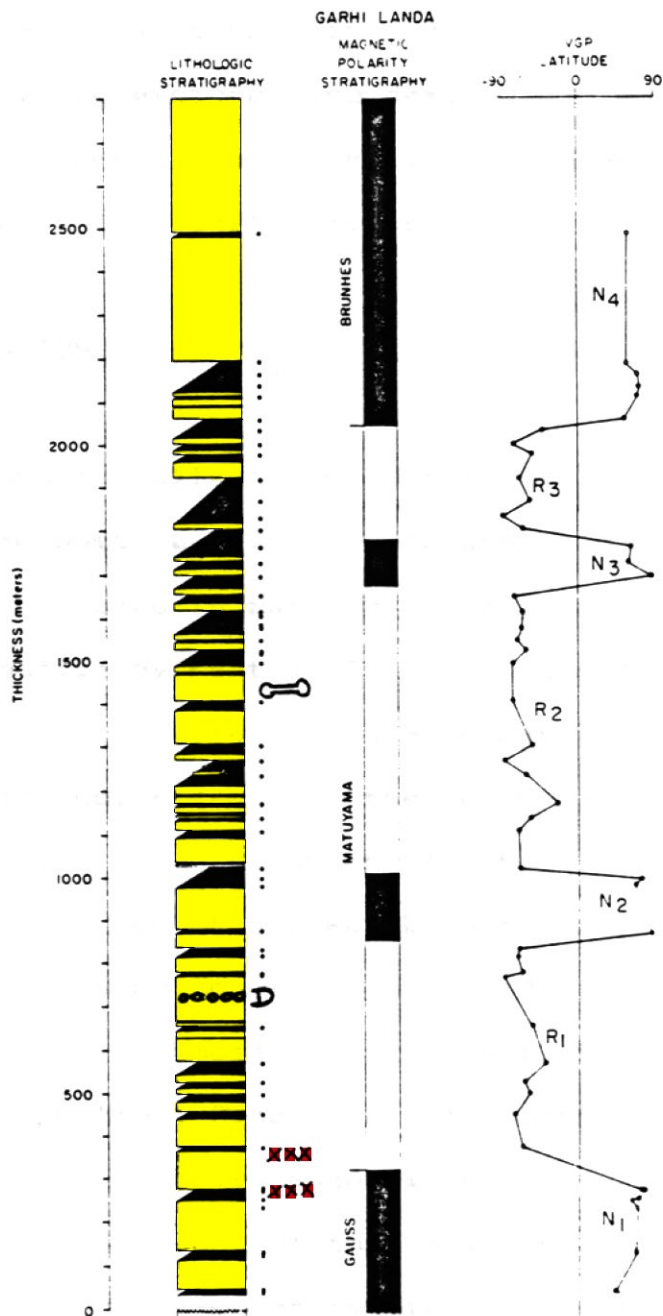
Fig. 3.10. Plot of VGP latitudes versus stratigraphic thickness. Plotting conventions are same as for Fig. 3.3. The bone symbol, Letter D, and xxx on the right side of the lithologic stratigraphic column mark location of the Stegodon fossils, the Bain Boulder Bed, and the ash units, respectively.
