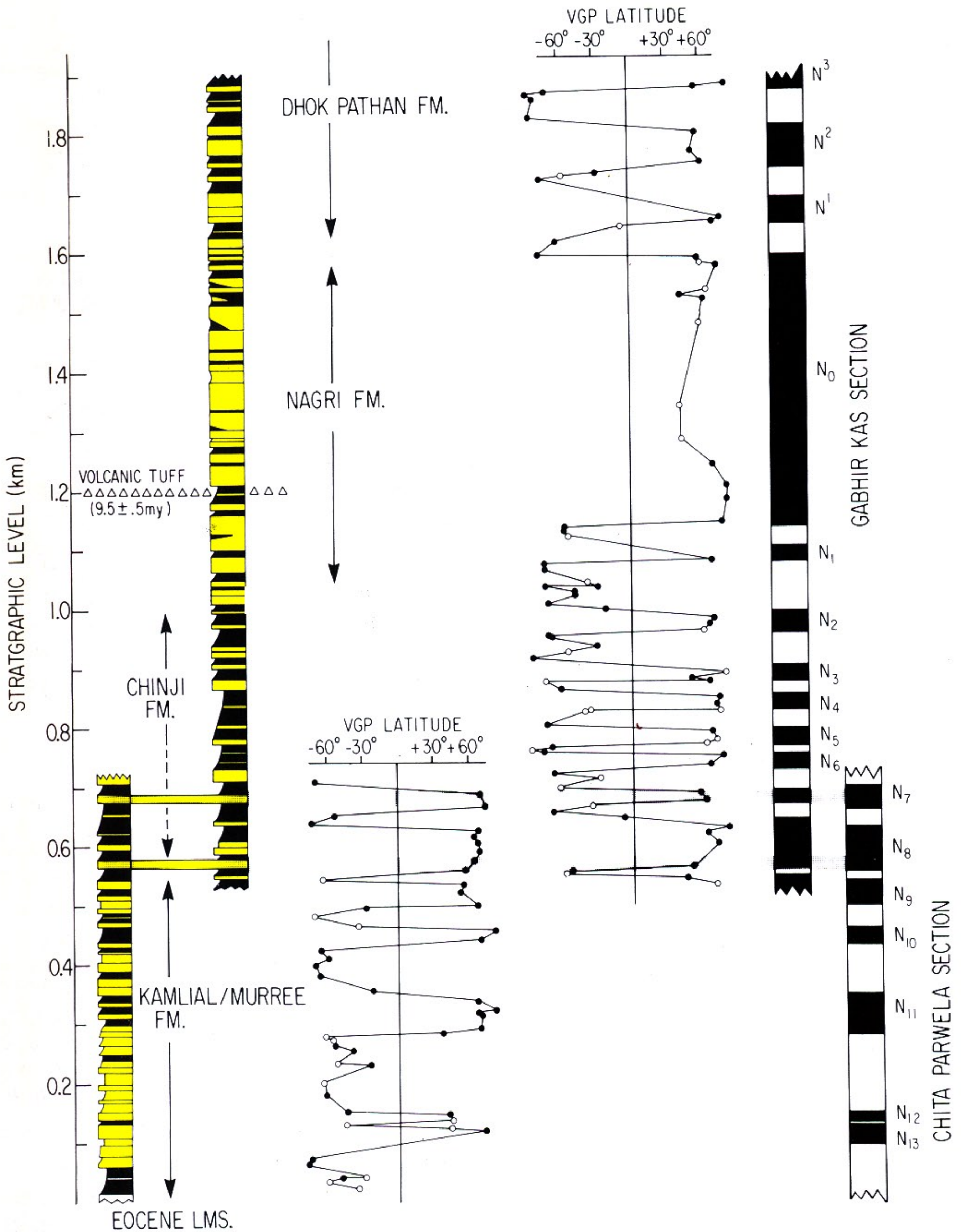
FIG. 4.—Superposition and magnetic polarity of sites in Chita Parwela section and Gabhir Kas section. Class A sites depicted as closed circles, class B as open circles. Tracer units between Chita Parwela and Gabhir Kas sections highlighted with shaded pattern.
