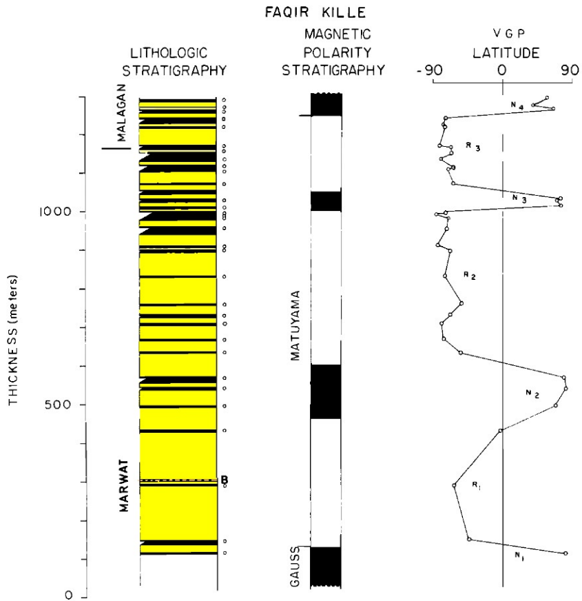
Fig. 10. Faqir Kille. Plot of VGP latitudes versus stratigraphic thickness. Plotting conventions are same as for Figure 6.
