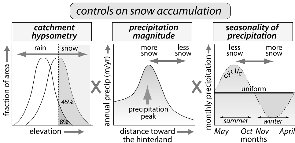
Figure 17. Conceptual summary of the three dominant factors exerting control on snow accumulation and hence snowmelt generation in mountainous regions: (1) Catchment hypsometry or elevation distribution within a catchment, (2) spatial distribution of precipitation magnitude, (3) seasonality or temporal distribution of precipitation. Higher topography, greater proximity to the precipitation peak, and a higher fraction of winter precipitation all lead to more snow accumulation.
