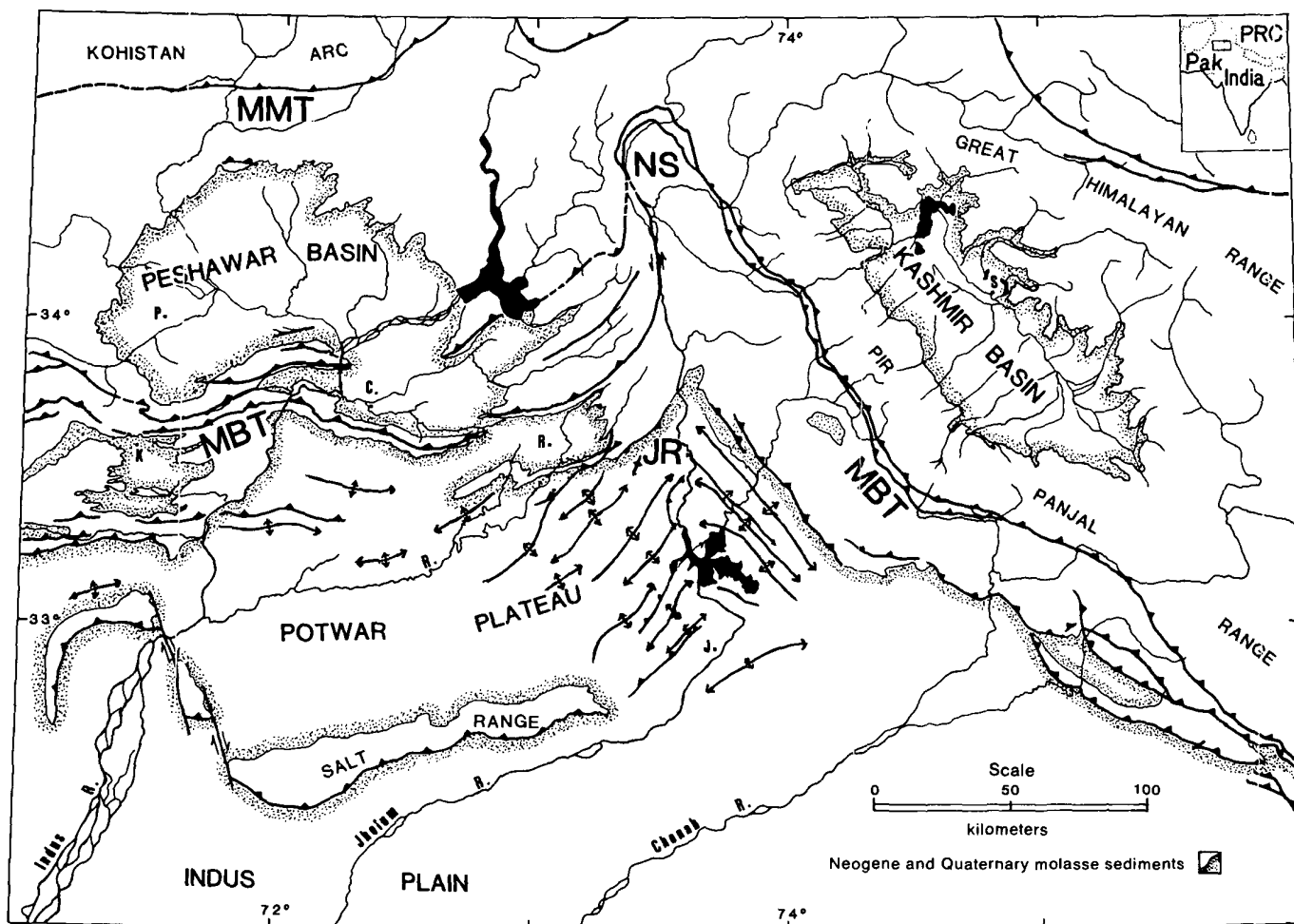
Figure 1. Map of the southern margin of the Himalaya and Hindu Kush. The Peshawar and Kashmir intermontane basins are symmetrically oriented about the Northwest Syntaxis (NS) and lie along the northern edge of the bounding Himalaya foredeep. C = Campbellpore; J = Jhelum; JR = Jhelum Re-entrant; K = Kohat; MBT = Main Boundary Thrust complex; MMT = Main Mantle Thrust; P = Peshawar; R = Rawalpindi; S = Srinagar.
