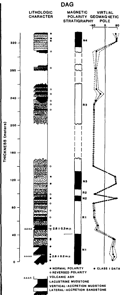
Figure 7. Magnetic-polarity stratigraphy from Dag. Stratigraphic locations of magnetic sites are indicated adjacent to the lithologic column. VGP latitudes form the basis for the magnetic zonation. The dashed lines define an alpha-95 error envelope on the VGP latitude determined for Class I sites. The ages (with a 2\sigma error) of volcanic ashes dated via the fission-track method are shown in their stratigraphic positions. These ages indicate that the N1/R1 transition is very likely to be the Gauss/Matuyama boundary. N3 is interpreted as the Olduvai subchron, N2 as one of the Reunion subchrons, and N4 as the lower part of the Brunhes chron.
