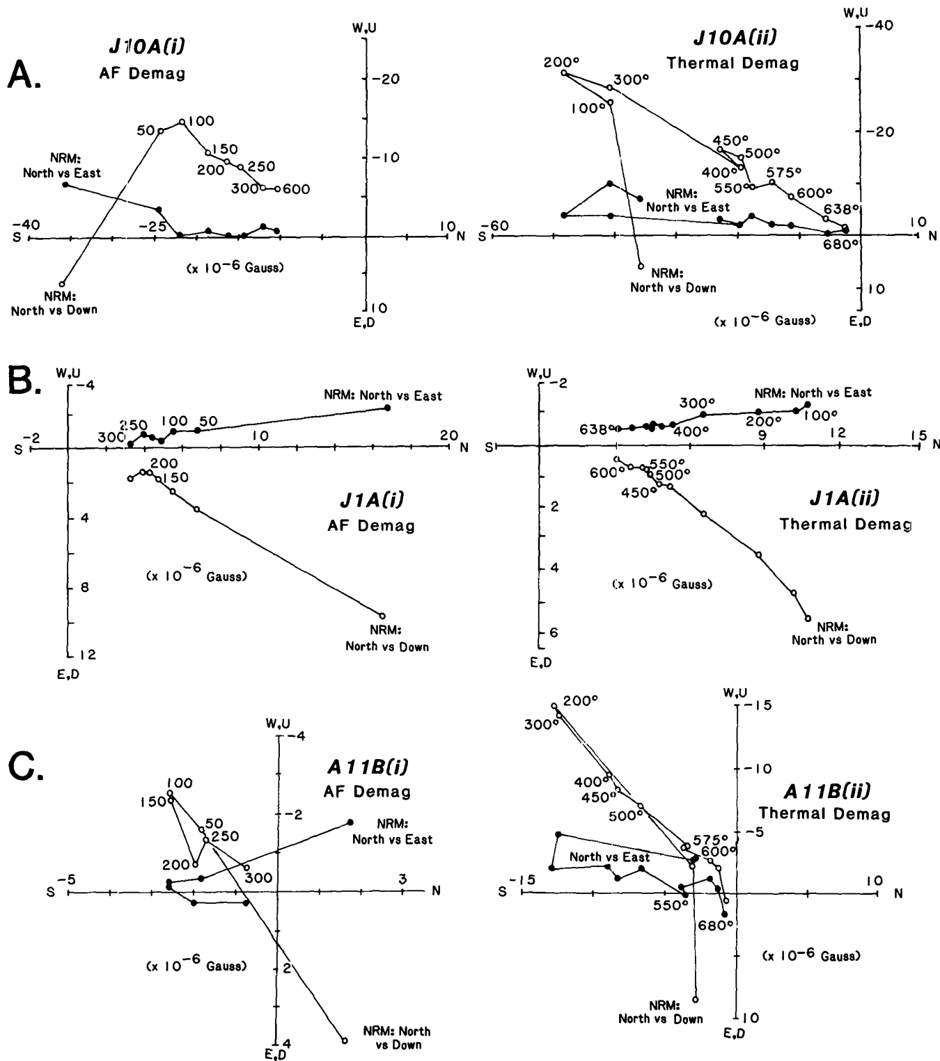
Figure 3. Zijdeveld plots comparing results of alternating-field and thermal demagnetization on adjacent, paired samples from Dag (A and B) and from Garhi Chandan (C). The numbers adjacent to the data points in the left-hand plots indicate the peak demagnetizing field in oersteds. The NRM directions after low levels of demagnetization (100 oe or 200 °C) are not significantly different between each set of paired samples for either of the demagnetization procedures.
