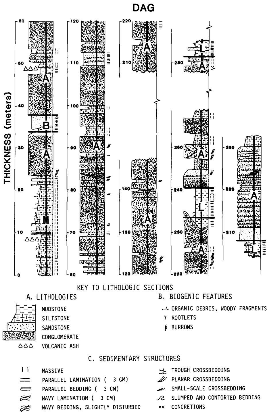
Figure 6. Lithologies and interpreted depositional environments from the Dag section. Three covered intervals occur between 145 and 305 m. A = alluvial fan, B = braided river, L = lacustrine, M = meandering river and floodplain. Above 23 m, alluvial fan conglomerates dominate the section as tectonically controlled fans prograded northward across the southern edge of the Peshawar basin behind the newly uplifted Attock Ranges.
