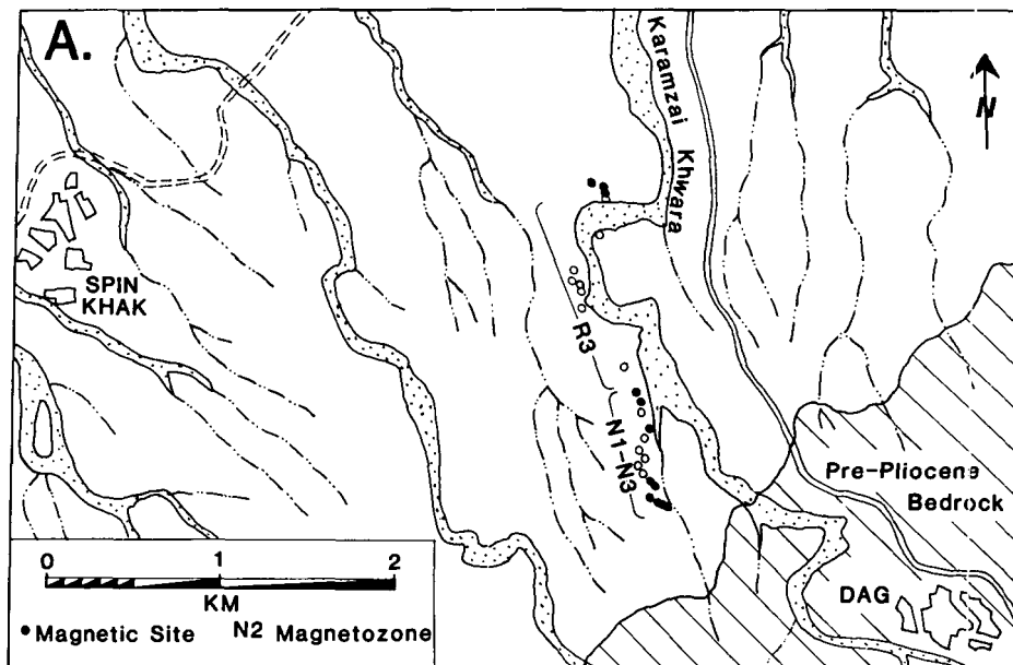
Figure 5A. Location map of the measured section at Dag based on Survey of Pakistan 1:63,360 topographic quadrangle (0/13, 1949). Magnetic-sampling sites and magnetozones are indicated.
