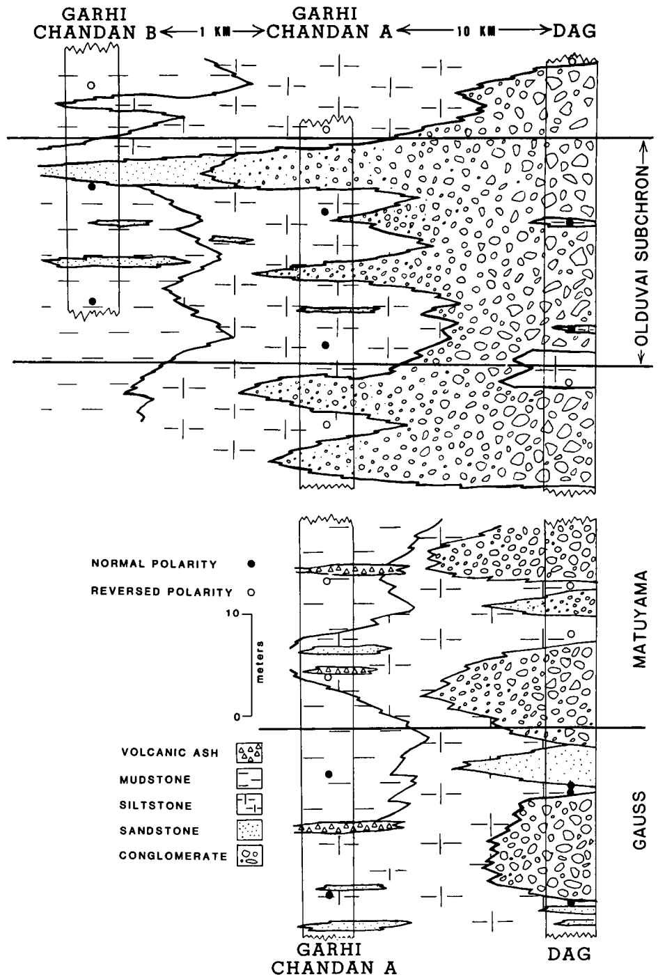
Figure 11. Time-transgressive facies relationships illustrated from dated sections at Dag and Garhi Chandan. Correlations between the sections are based on isochronous magnetic boundaries interpreted to be encompassed by each section. Around 2.5 m.y. ago, alluvial-fan sedimentation is confined to the more proximal Dag area, while lacustrine mudstones and low-energy fluvial sandstone and siltstone facies dominate the more distal Garhi Chandan area. Around the Olduvai subchron, 700,000 yr later, the distal fan facies have prograded sufficiently to cover intermittently the more proximal Garhi Chandan area with coarse conglomerates. However, rapid facies transitions occur between Garhi Chandan sections A and B such that only low-energy deposition is recorded in the more distal sequence despite the coarse conglomerates 1 km farther south.
