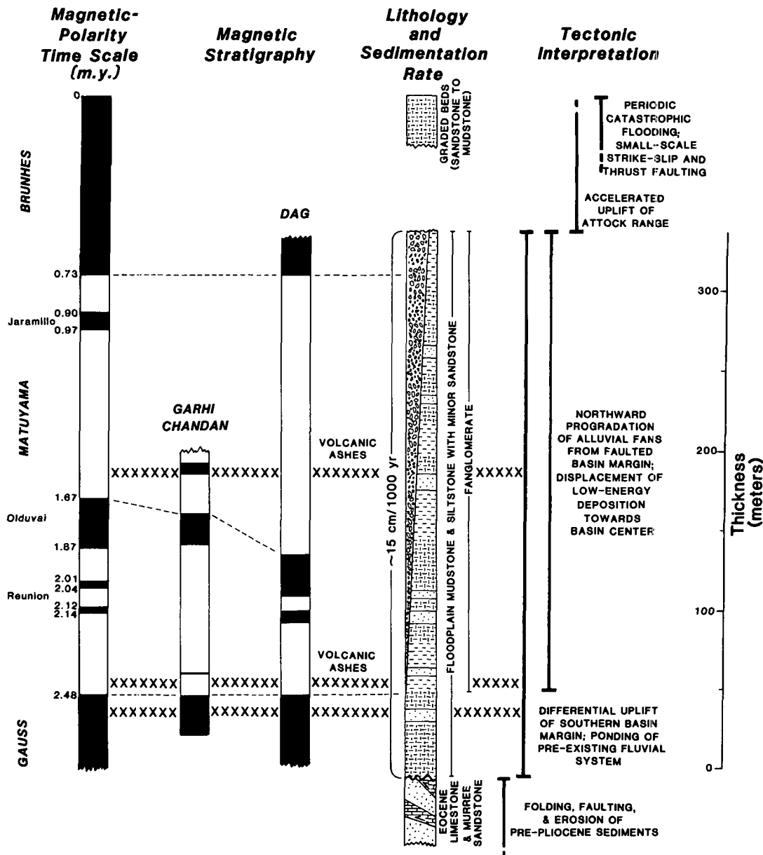
Figure 12. Summary diagram of the chronologic and stratigraphic data from the Peshawar basin. A tectonic interpretation of the lithofacies is presented on the right. Intermontane-basin development is initiated by differential uplift of the ancestral Attock Range. The resultant ponding of fluvial sediments within the Peshawar basin begins in the late Pliocene and continues through much of the Pleistocene. During this interval, tectonically modulated fanglomerates prograde northward across the basin margin and gradually displace the lower-energy environments toward the basin center. Accelerated uplift of the Attock Range terminated widespread intermontane-basin deposition after 600,000 yr ago. Subsequently, the catastrophic floods have periodically inundated the basin, and recent faulting has disrupted young, basin-filling sediments.
