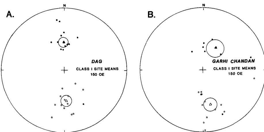
Figure 4. Stereonet plot of the mean directions of Class I sites from (A) Dag and (B) Garhi Chandan. The sites from each area plot generally antipodally and pass the reversal test. They also suggest that there has been no significant postdepositional tectonic rotation of these areas.
