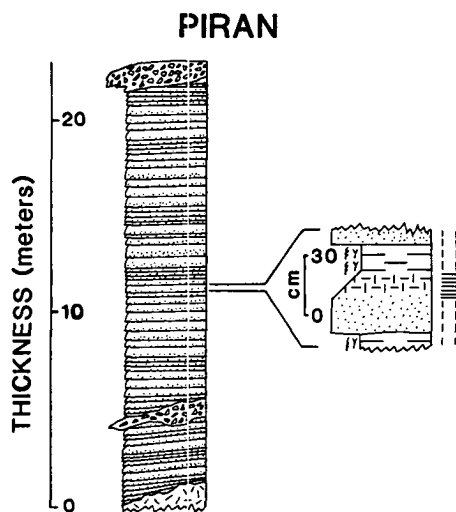
Figure 10. Measured section of cyclical sediments at Piran. Lithologies and sedimentary structures of a typical depositional unit are illustrated at the right. Below the colluvial zone at 4 m, the beds dip to the north at 10^\circ , whereas above it, they dip at only 2^\circ to the north.
