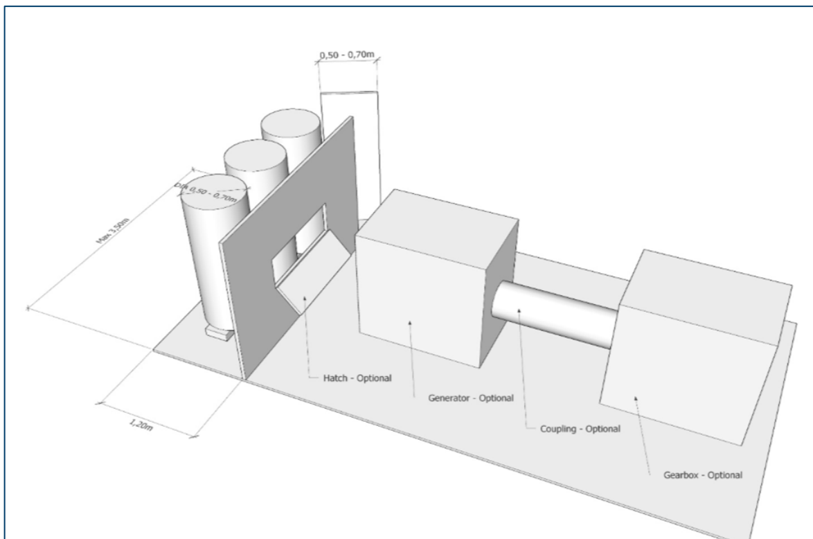
Figure 6-32 - Recommended dimensions for the Nacelle Mock-up
