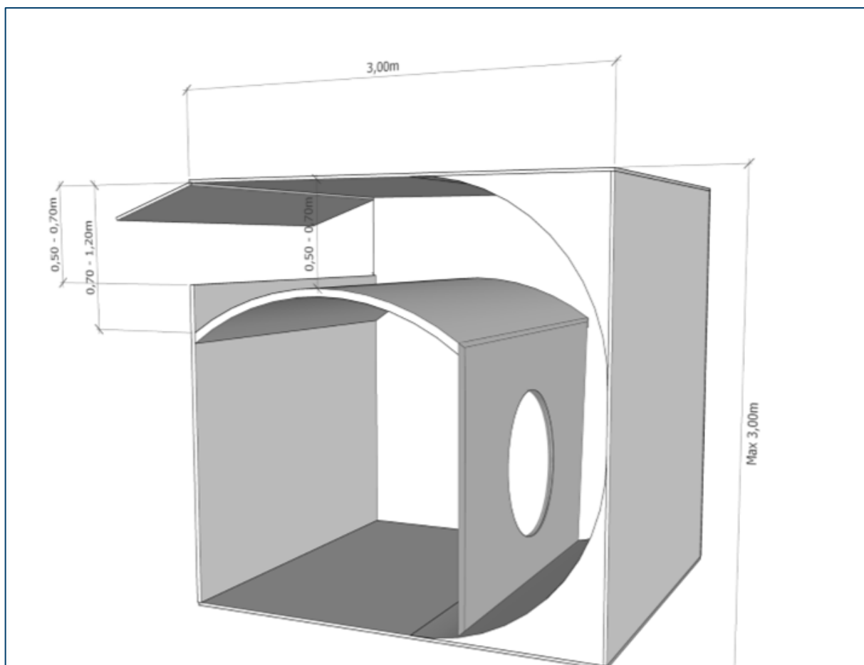
Figure 6-31 - Recommended dimensions for the Hub Mock-up
