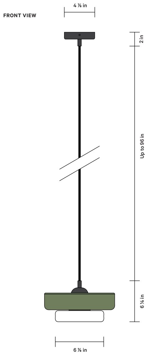
FRONT VIEW
