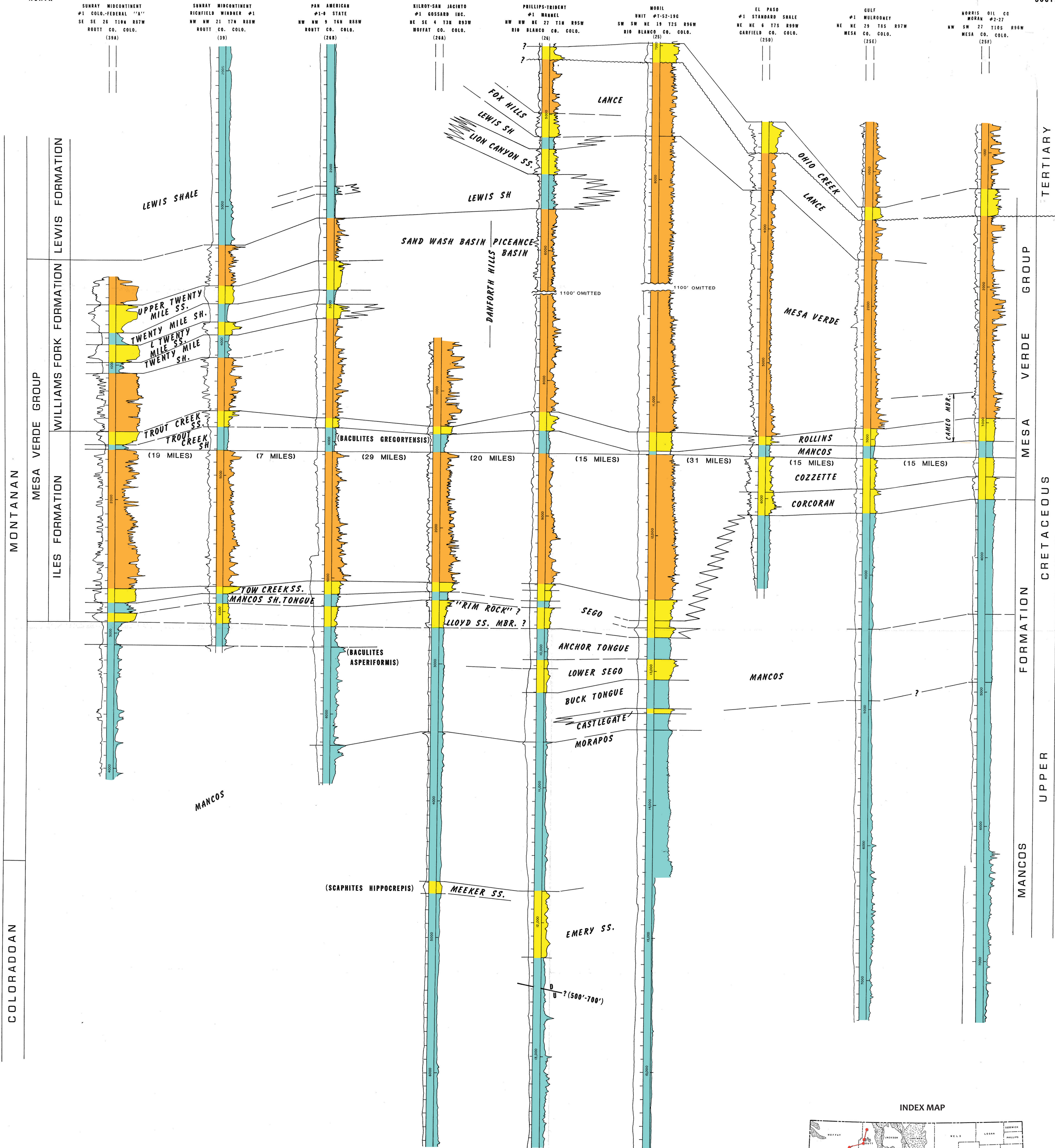
SAND WASH & PICEANCE BASIN COLORADO UPPER CRETACEOUS ROCKS SUBSURFACE CORRELATION
