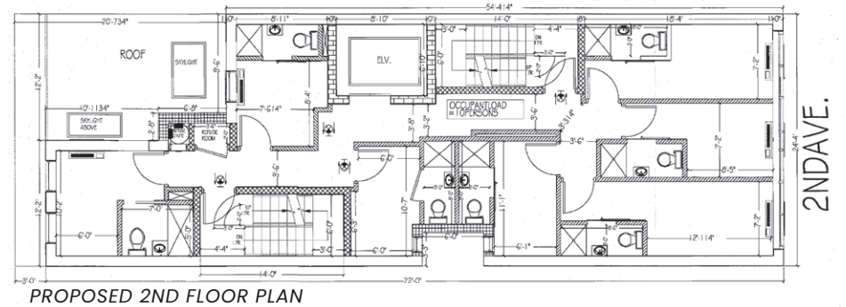
PROPOSED 2ND FLOOR PLAN
