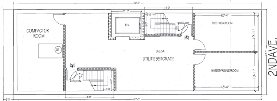
PROPOSED CELLAR FLOOR PLAN
