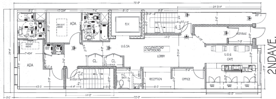
PROPOSED 1ST FLOOR LOBBY PLAN
