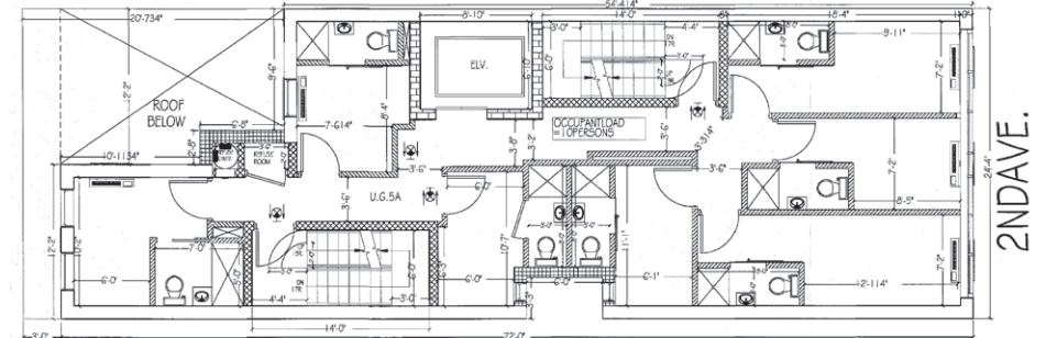
PROPOSED 3RD-5TH FLOOR PLAN
