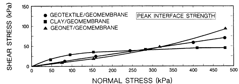
FIG. 10. Peak Failure Envelopes for Various Liner Interfaces
