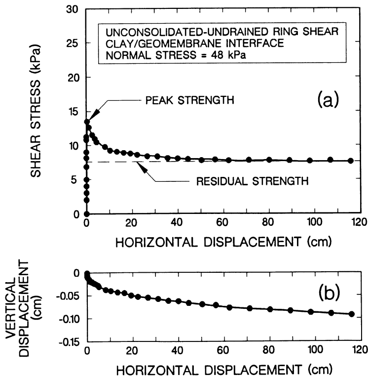
FIG. 3. Typical Undrained Ring-Shear Test Results for Secondary Clay/Secondary Geomembrane Interface: (a) Shear Stress; (b) Vertical Displacement
