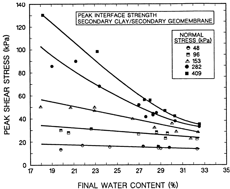
FIG. 5. Peak Secondary Clay/Secondary Geomembrane Interface Strengths
