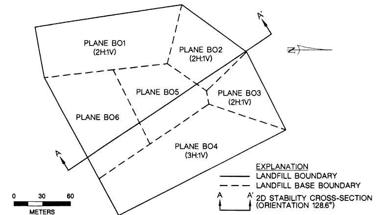
FIG. 13. Kettleman Hills Landfill B-19, Phase IA Geometry for Stability Analyses (after Byrne et al. 1992)
