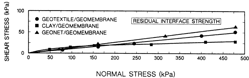
FIG. 11. Residual Failure Envelopes for Various Liner Interfaces
