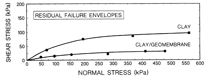
FIG. 9. Comparison of Residual Clay and Residual Clay/Geomembrane Interface Strengths
