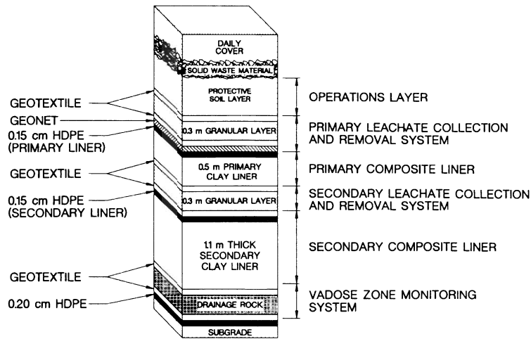
FIG. 1. Composite Double-Liner System at Base of Landfill (from Mitchell et al. 1990)
