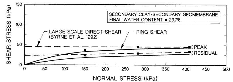
FIG. 7. Undrained Secondary Clay/Secondary Geomembrane Interface Failure Envelopes
